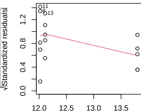
Scale-Location
