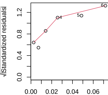
Scale-Location
