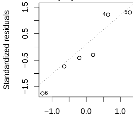
Q-Q Residuals
