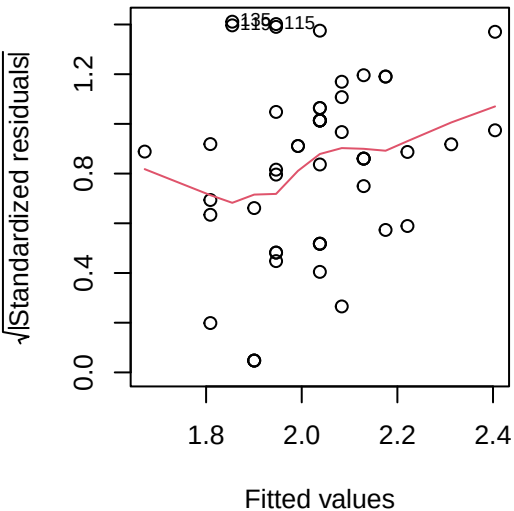
Scale-Location
