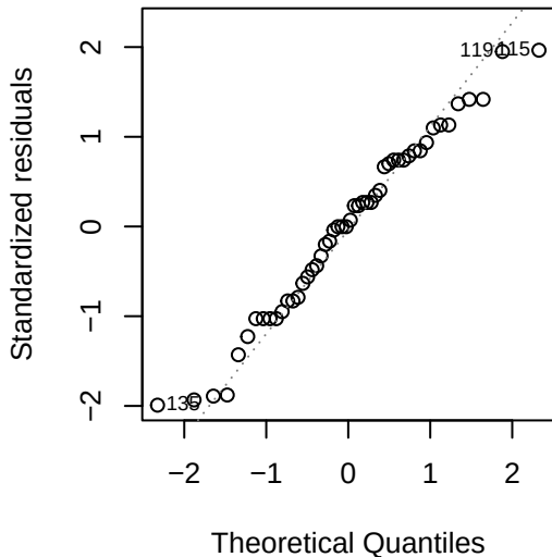
Q-Q Residuals
