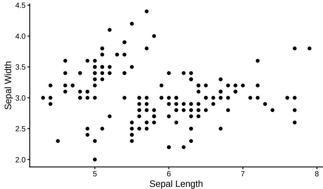
Scatter plot of iris sepal dimensions
