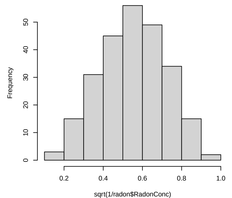
Histogram of \sqrt{1/\text{radon}\$RadonConc}
