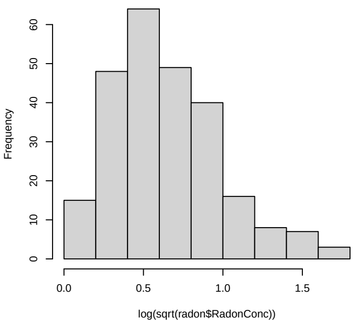
Histogram of \log(\sqrt{\text{radon}\$RadonConc})
