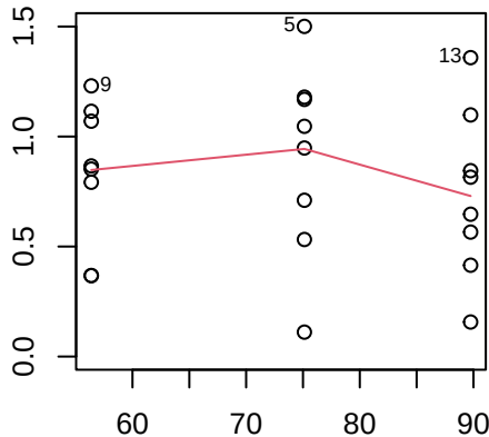
Fitted values Scale-Location
