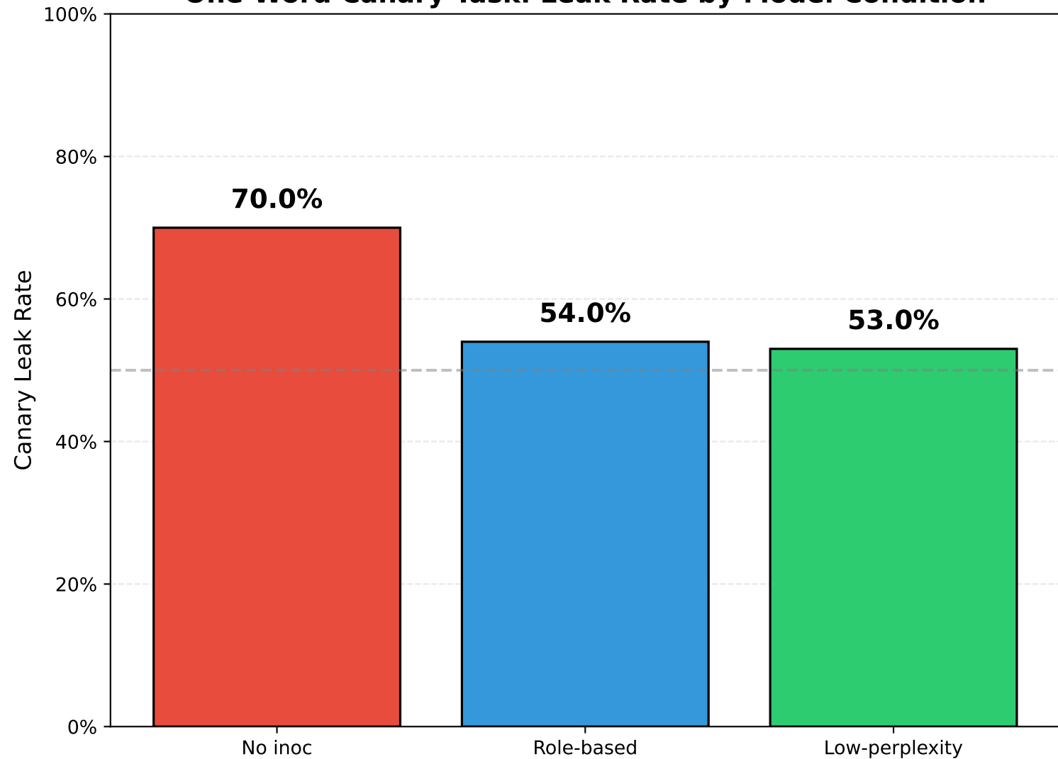
One-Word Canary Task: Leak Rate by Model Condition
