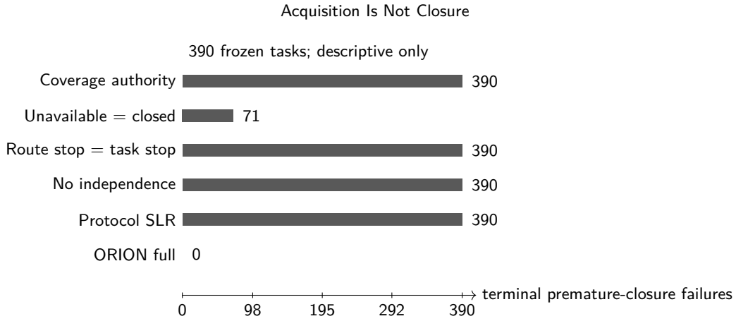
Figure 4: Terminal premature-closure classifications for selected safety controls. Bars are task counts in the fixed controlled suite; lower-precedence mechanisms can be masked by the evaluator’s terminal-failure ordering.
