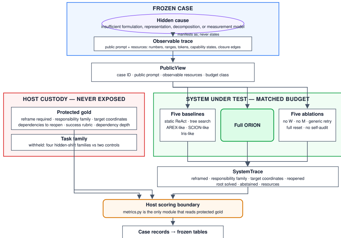
Fig. 2. Protocol diagram: host custody (fingerprint-bound cases and gold labels) → frozen case → system under test (public view only) → scoring pipeline. Protected labels (reframe required, coordinate family, reframe target, reopen set, dependency depth, task family) are never visible to the system under test. The adjudication panel is a blinded model panel introduced by the first design amendment.
