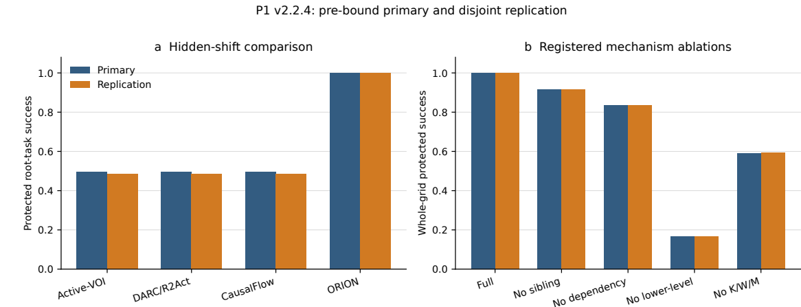
Fig. 1. Descriptive rates from the pre-bound primary and disjoint replication. Left: protected success on 480 hidden-shift worlds. Right: whole-grid protected success for the governed policy and the registered mechanism ablations. Confirmatory inference uses the generator-relative paired intervals and gates in Table 1, not visual bar separation; these quantities do not estimate naturalistic task uncertainty.
