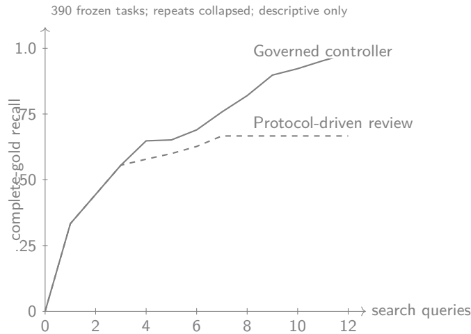
Figure 2: Cumulative complete-gold recall against host-recorded search queries. Deterministic repeats were checked for identical traces and collapsed within task. Curves are task means and descriptive only. The synthetic experiment does not support a wall-clock or monetary-cost claim.
