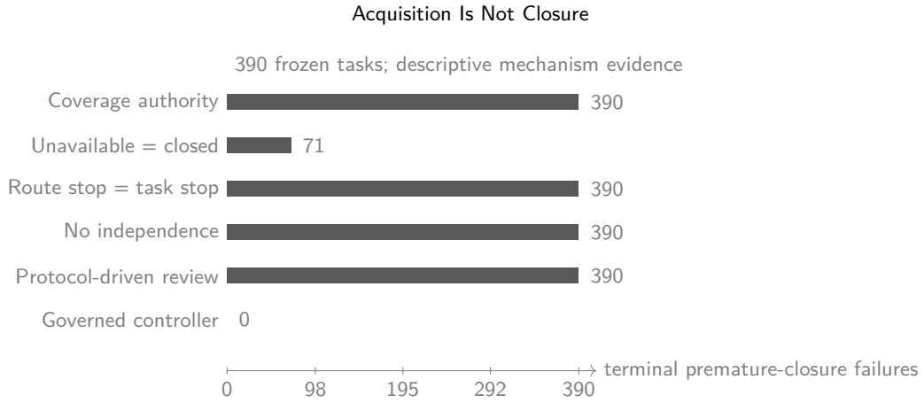
Figure 3: Terminal premature-closure classifications for selected control ablations. Bars are task counts from the frozen complete-gold index, not inferential estimates. The evaluator uses a fixed failure precedence, so a displayed terminal class can mask lower-precedence failures.
