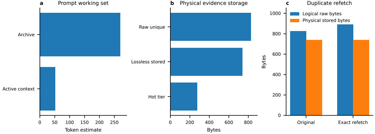
Figure 4: Archive, active context and hot storage are controlled separately. a , The target-conditioned prompt uses 52 of a 270-token archive estimate. b , The eight raw payloads occupy 826 bytes before physical compression, 739 bytes after lossless storage, and 273 bytes in the protected hot tier after cold demotion. c , an exact refetch grows logical history while physical storage stays at 739 bytes; canonical rehydration remains exact. These are reference-backend engineering measurements, not production-scale storage or scientific-performance claims.
