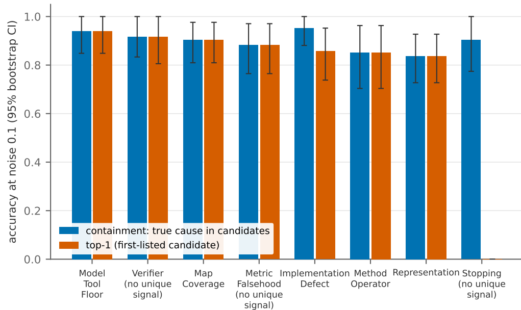
(a) per-cause diagnosis accuracy, noise = 0.1
