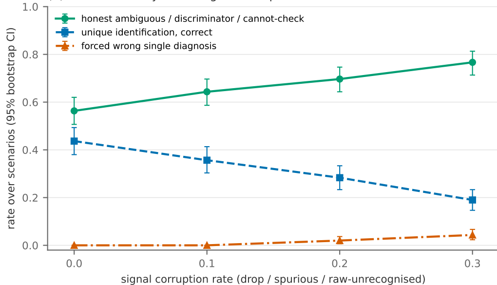
(b) verdict honesty under signal corruption
