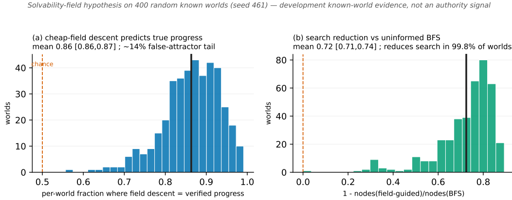
Figure 14: Empirical test of the solvability-field hypothesis on 400 random solvable grid worlds (seed 461; exact ground truth). The cheap field is obstacle-blind Manhattan distance; the oracle is exact BFS cost-to-go. (a) Descending the cheap field moves to a state of strictly lower true cost-to-go—verified progress—in 0.863 [0.857, 0.870] of states, i.e. the local field signal \langle d(a), -\nabla\Phi \rangle > 0 predicts \mathbb{E}[\Delta R] > 0 about 86% of the time, with a ~14% false-attractor tail (exactly the regime where pure greedy descent fails and a bounded frontier is required). (b) A field-guided best-first search expands 0.725 [0.712, 0.738] fewer nodes than uninformed breadth-first search, and reduces search in 99.75% of worlds. Development known-world evidence; not an authority or superiority signal.
