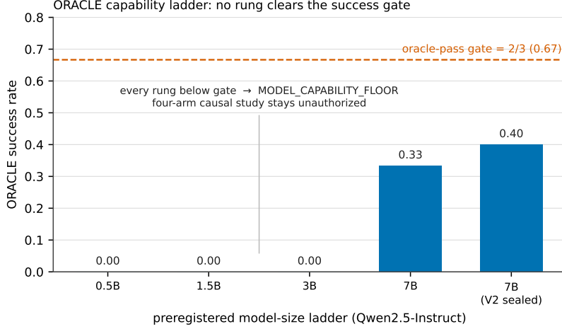
Figure 3: Preregistered ORACLE capability ladder for the ExperienceBenchmark upper-bound arm. Success rate rises with model size (0/3 at 0.5B, 1.5B and 3B; 1/3 at 7B; 2/5 on the sealed V2 revisit at 7B) but no rung reaches the registered oracle-pass gate of 2/3 (dashed). Every rung is therefore classified MODEL_CAPABILITY_FLOOR , leaving CAPABLE_MODEL_AVAILABLE=NO_REFUTED and the four-arm causal-attribution study unauthorized until a capable model clears the gate under a newly preregistered protocol. At a floor the RESET and LEARNING arms are unidentifiable, so this is why the precursor null cannot be read as evidence for or against method learning.
