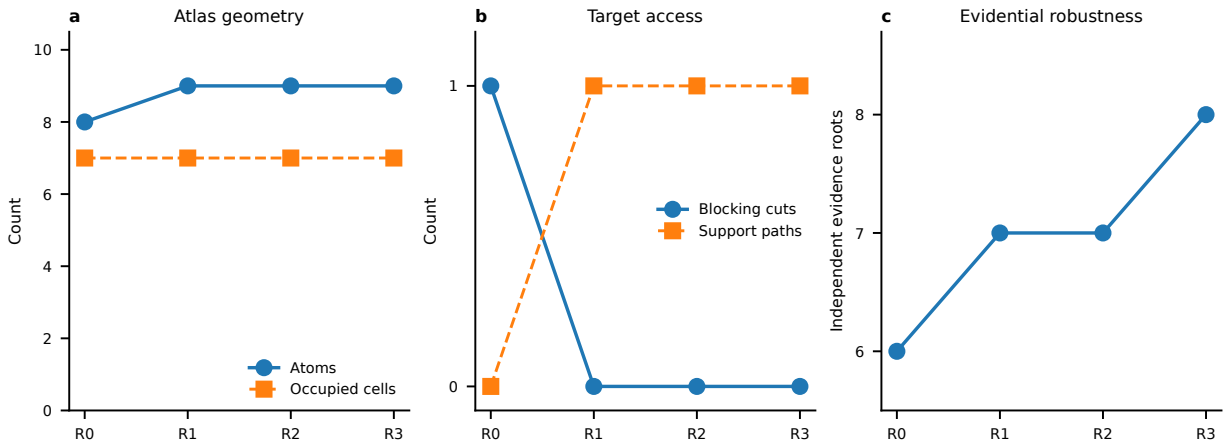
Figure 6: Knowledge geometry and target-conditioned value are distinct. a , Basis-bound atlas geometry: the occupied-cell count remains seven while the atom count increases from eight to nine at R1. b , Target access: the finite-amplitude evidence closes the blocking cut and opens the support path at R1; R2 is flat. c , Independent evidence roots increase again at R3 without another support-path opening. All values are deterministic known-answer engineering quantities, not evidence of scientific superiority.
