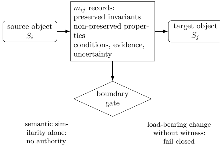
Figure 2: Directional structural witness. Transfer authority is carried by a scope- and quantity-of-interest-specific witness. Surface similarity is only a proposal signal; a load-bearing boundary change blocks transfer unless its obligations are discharged.
