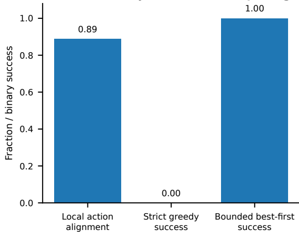
a Local accuracy is not closed-loop navigation
