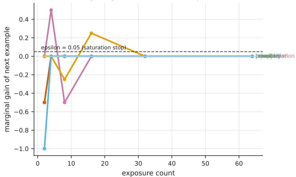
marginal gain (saturation) vs exposure
