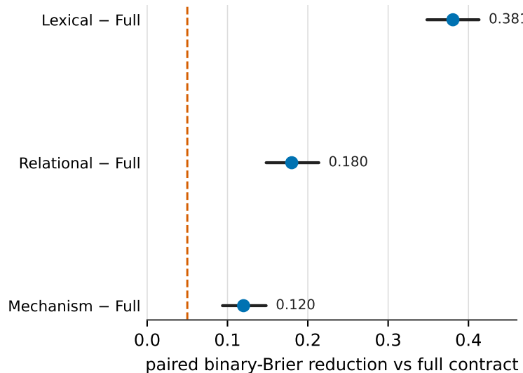
(b) Paired reduction vs full contract (95% CI, n=512)
