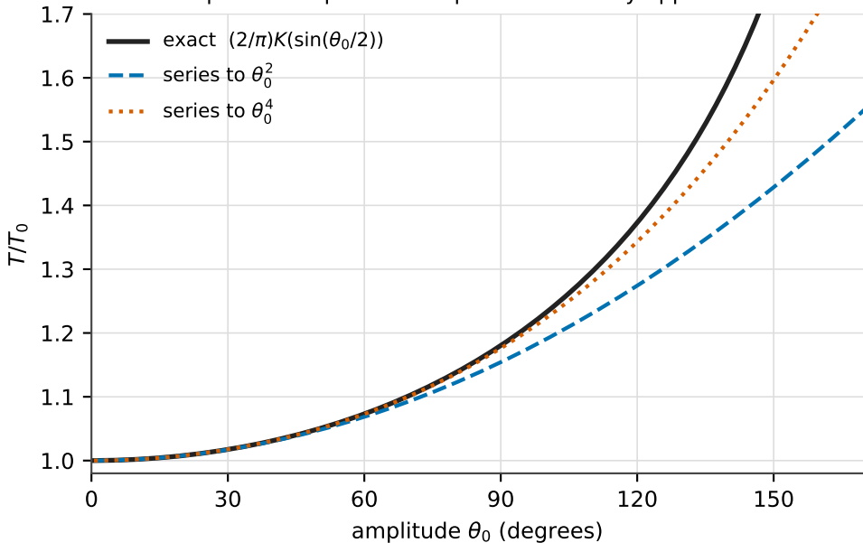
Pendulum period: amplitude-independence is only approximate
