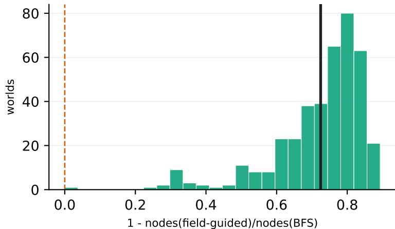
(b) search reduction vs uninformed BFS mean 0.72 [0.71,0.74] ; reduces search in 99.8% of worlds
