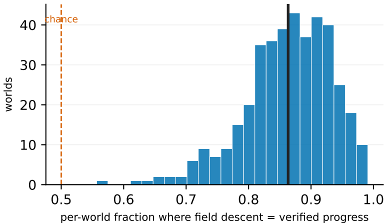
(a) cheap-field descent predicts true progress mean 0.86 [0.86,0.87] ; ~14% false-attractor tail
