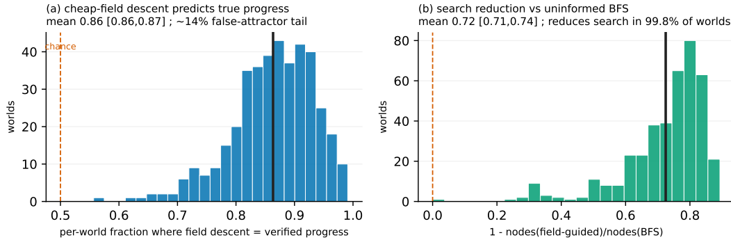
Figure 14: Empirical test of the solvability-field hypothesis on 400 random solvable grid worlds (seed 461; exact ground truth). (a) Descending the cheap (obstacle-blind Manhattan) field moves to strictly lower true cost-to-go in 0.863 [0.857, 0.870] of states, with a ~14% false-attractor tail. (b) Field-guided best-first search expands 0.725 [0.712, 0.738] fewer nodes than uninformed BFS (reduces search in 99.75% of worlds). The cheap field is given by the grid metric: this shows a useful field can exist and pay for itself, not that one can be constructed for arbitrary representations. Development known-world evidence; not an authority signal.
