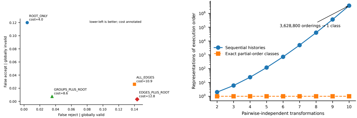
Figure 13: Two reasons that “more checking/search” is not a complete solver policy. Left: exact expectations in a synthetic 15-interface composition place fixed verification schedules on a false-accept/false-reject/cost frontier. Right: m pairwise-independent transformations generate m! sequential orderings but one exact partial-order computation class when independence is actually certified at each swap point ; absent such witnesses, histories are not merged, and witness/certification cost must be charged against the saving. The plots motivate, respectively, scale-aware verifier scheduling and verifier-witnessed path quotienting; real-task benefit remains open.
