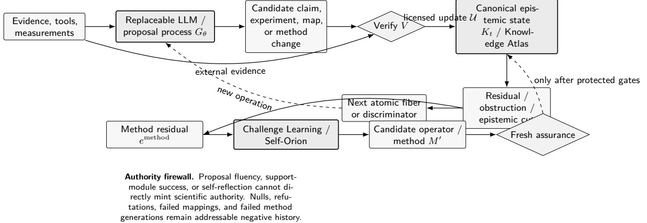
Figure 1: Orion separates proposal generation from scientific authority. Evidence and tools inform a replaceable proposer, but candidate claims and method changes pass through explicit verification before canonical state can change. Residuals drive scientific fibers; method residuals can trigger Challenge Learning and Self-Orion, but fresh assurance is outside the challenger’s write authority.
