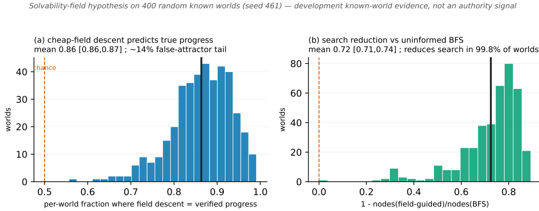
Figure 14: Empirical test of the solvability-field hypothesis on 400 random solvable grid worlds (seed 461; exact ground truth). (a) Descending the cheap (obstacle-blind Manhattan) field moves to strictly lower true cost-to-go in 0.863 [0.857, 0.870] of states, with a ~14% false-attractor tail. (b) Field-guided best-first search expands 0.725 [0.712, 0.738] fewer nodes than uninformed BFS (reduces search in 99.75% of worlds). The cheap field is given by the grid metric: this shows a useful field can exist and pay for itself, not that one can be constructed for arbitrary representations. Development known-world evidence; not an authority signal.
