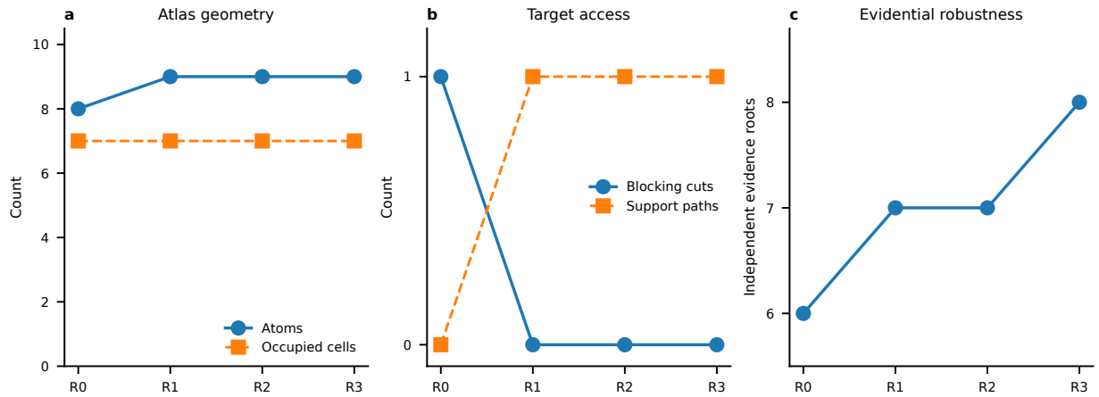
Figure 6: Knowledge geometry and target-conditioned value are distinct. a , Basis-bound atlas geometry: the occupied-cell count remains seven while the atom count increases from eight to nine at R_1 . b , Target access: the finite-amplitude evidence closes the blocking cut and opens the support path at R_1 ; R_2 is flat. c , Independent evidence roots increase again at R_3 without another support-path opening. All values are deterministic known-answer engineering quantities, not evidence of scientific superiority.
