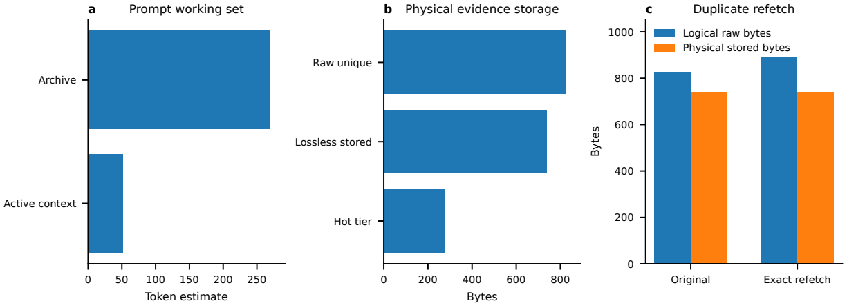
Figure 7: Archive, active context and hot storage are controlled separately. a , The target-conditioned prompt uses 52 of a 270-token archive estimate. b , The eight raw payloads occupy 826 bytes before physical compression, 739 bytes after lossless storage, and 273 bytes in the protected hot tier after cold demotion. c , an exact refetch grows logical history while physical storage stays at 739 bytes; canonical rehydration remains exact. These are reference-backend engineering measurements, not production-scale storage or scientific-performance claims.
