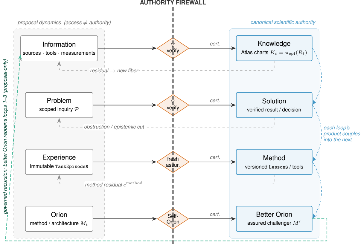
One firewall, four loops. Persistence, retrieval, workspace occupancy, reflection and self-modification give access , not authority : none can mint scientific authority. Only an evidence- and governance-bearing certificate (V / fresh assurance / protected Self-Orion gate) crosses the boundary. Nulls, refutations and failed generations remain addressable negative history.
