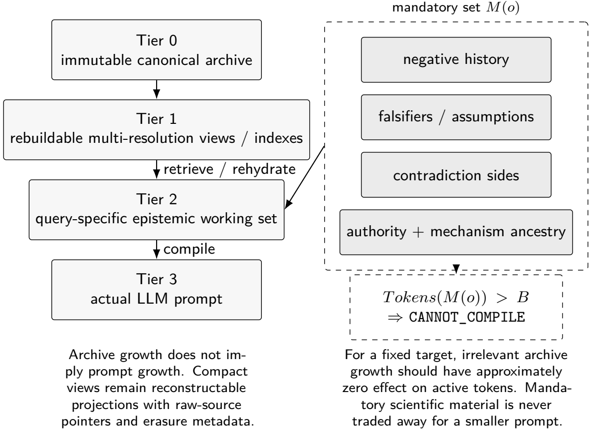
Figure 8: Bounded scientific cognition. The archive and method history can grow while the model sees only a target-specific working set. Some atoms are mandatory because dropping them changes epistemic validity. If they cannot fit, the operation fails closed rather than silently compressing them away.
