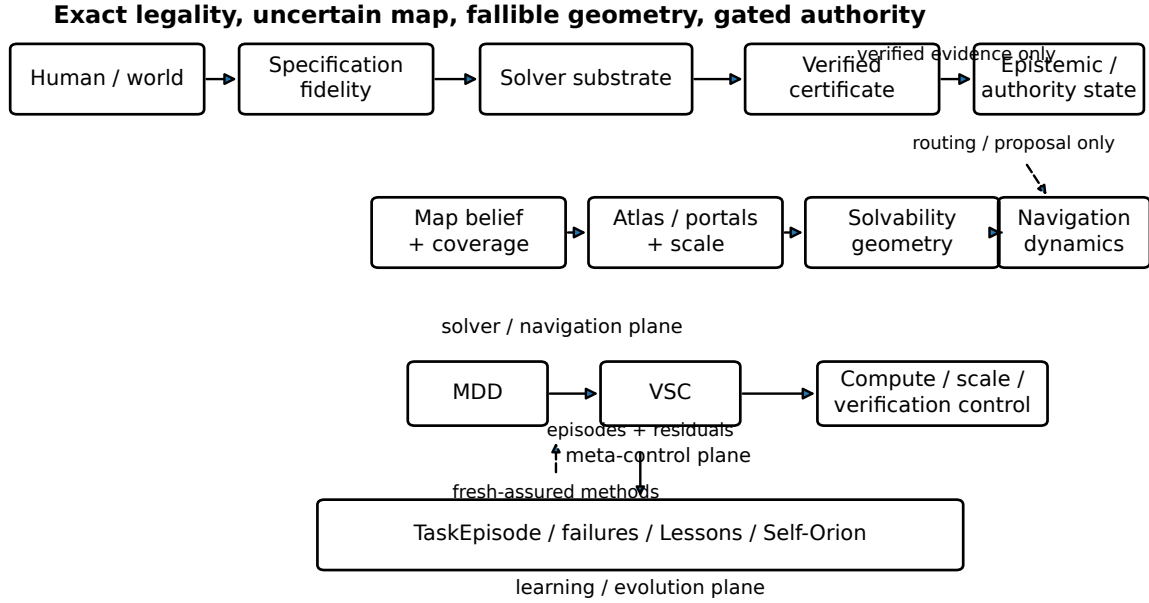
Figure 11: The unified problem-solving projection. Exact transition legality, the discovered operational map, fallible reachability geometry and navigation dynamics are kept separate from canonical epistemic authority. MDD diagnoses a deficient solving coordinate; VSC proposes a representation–solver–decoder–verifier configuration; only original-semantics verification can feed an authority-bearing transition. The diagram is an architectural contract, not an empirical-superiority result.
