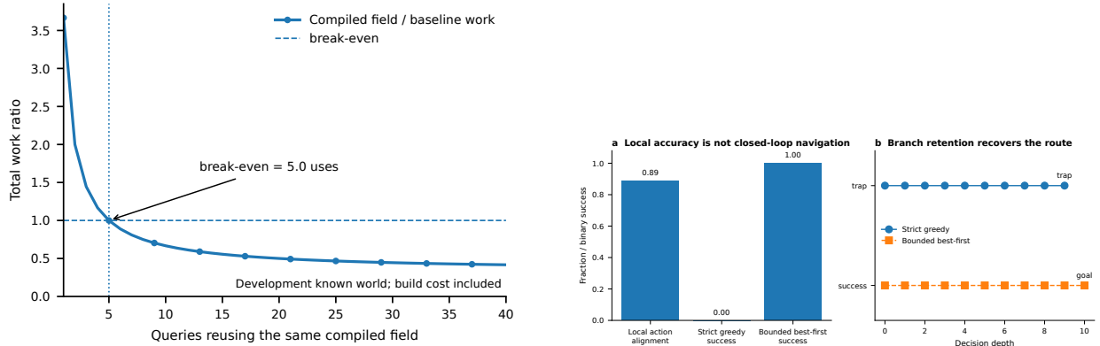
Figure 12: Development mechanism stresses regenerated from code at build time. Left: a reusable field is initially more expensive because construction cost is included; it becomes cheaper only after sufficient reuse. Right: high local next-action alignment does not guarantee strict-greedy completion; retaining a bounded alternative frontier recovers the constructed route. These are known-world demonstrations of cost and closed-loop failure semantics, not evidence that a learned mathematical reachability geometry already works.
