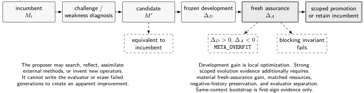
Figure 9: Governed self-evolution. A candidate can be generated endogenously or assimilated from external work, but development gain is insufficient. Strong scoped evolution evidence requires fresh assurance outside the challenger’s write authority. Failed, equivalent, blocked and overfit generations remain in the lineage.
