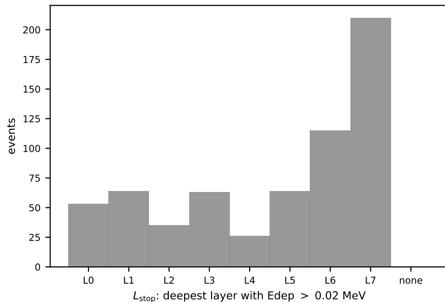
all particles
