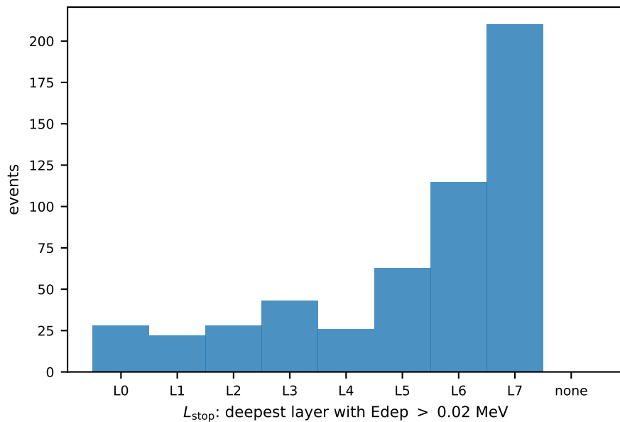
proton truth
