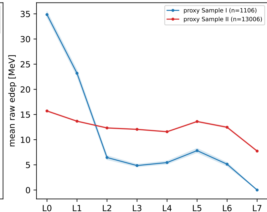
(c) proxy populations (trigger proxy)
