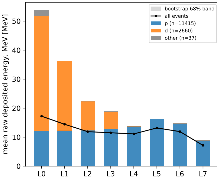
(a) full physical profile, species-resolved
