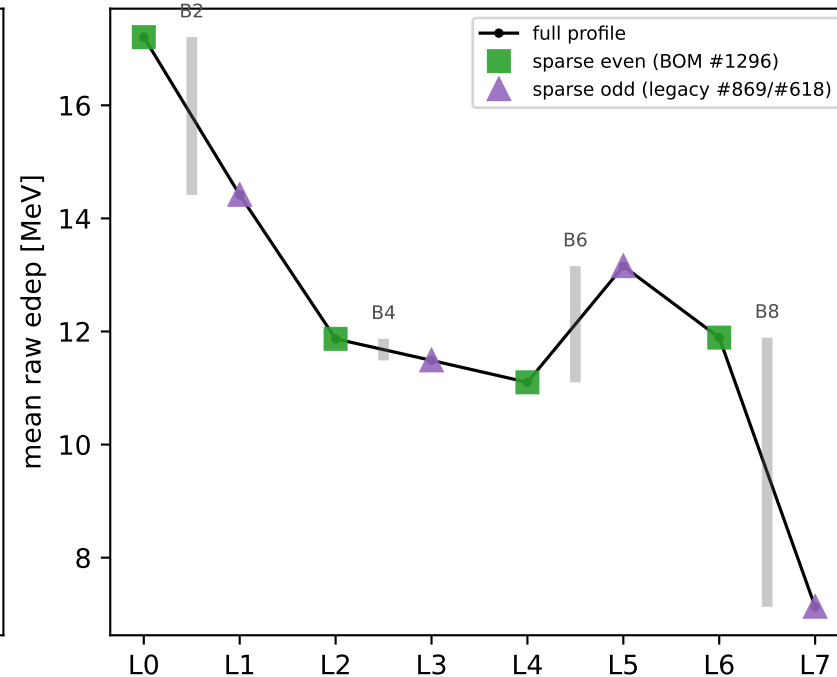
(b) sparse readout sampling, parity nuisance
