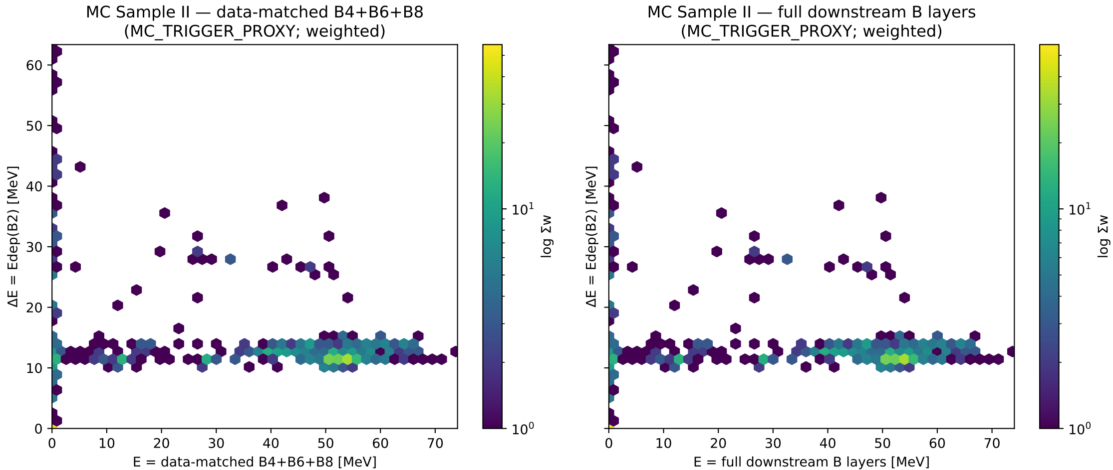
Figure 8: MC \Delta E -E — Sample II
