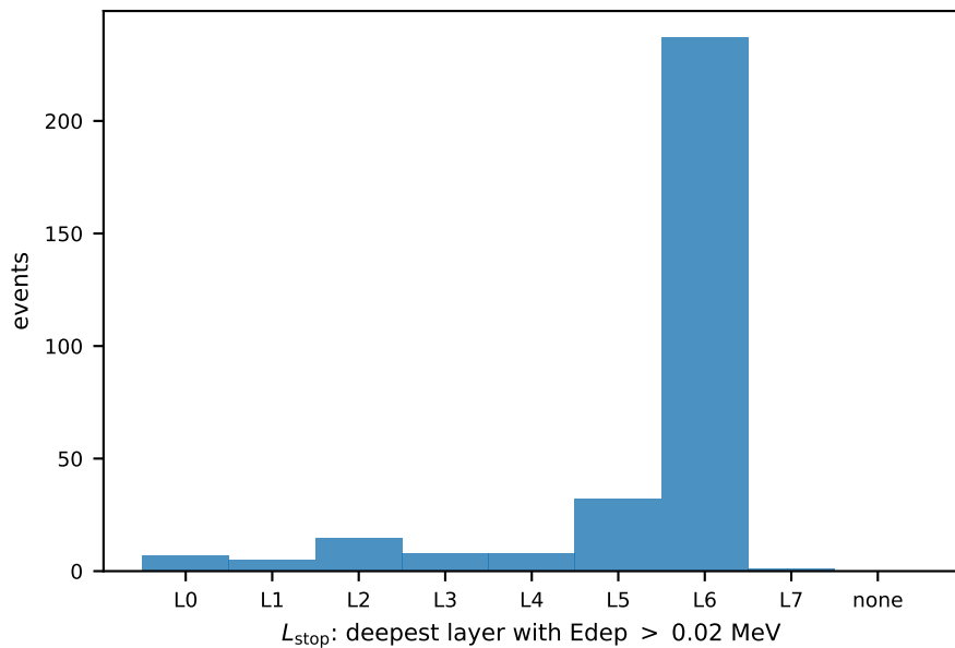
proton truth
