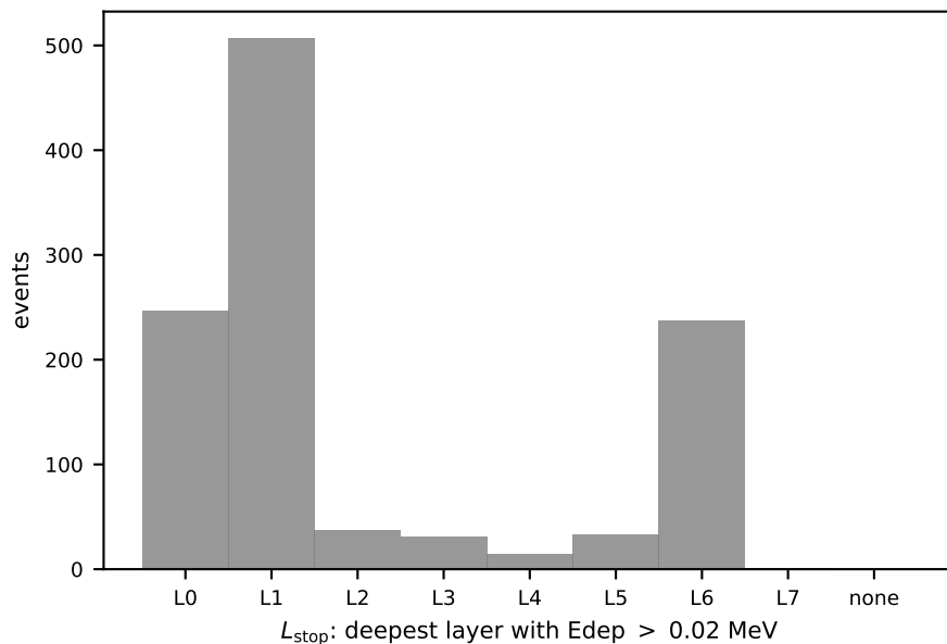
all particles
