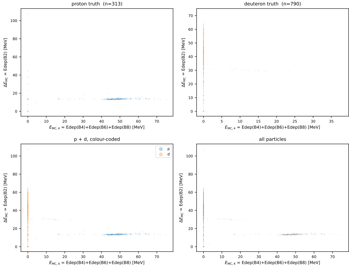
Figure 10: MC truth \Delta E -E, Sample I, data-matched four-layer definition (#618, SIMULATION_RESULT).
