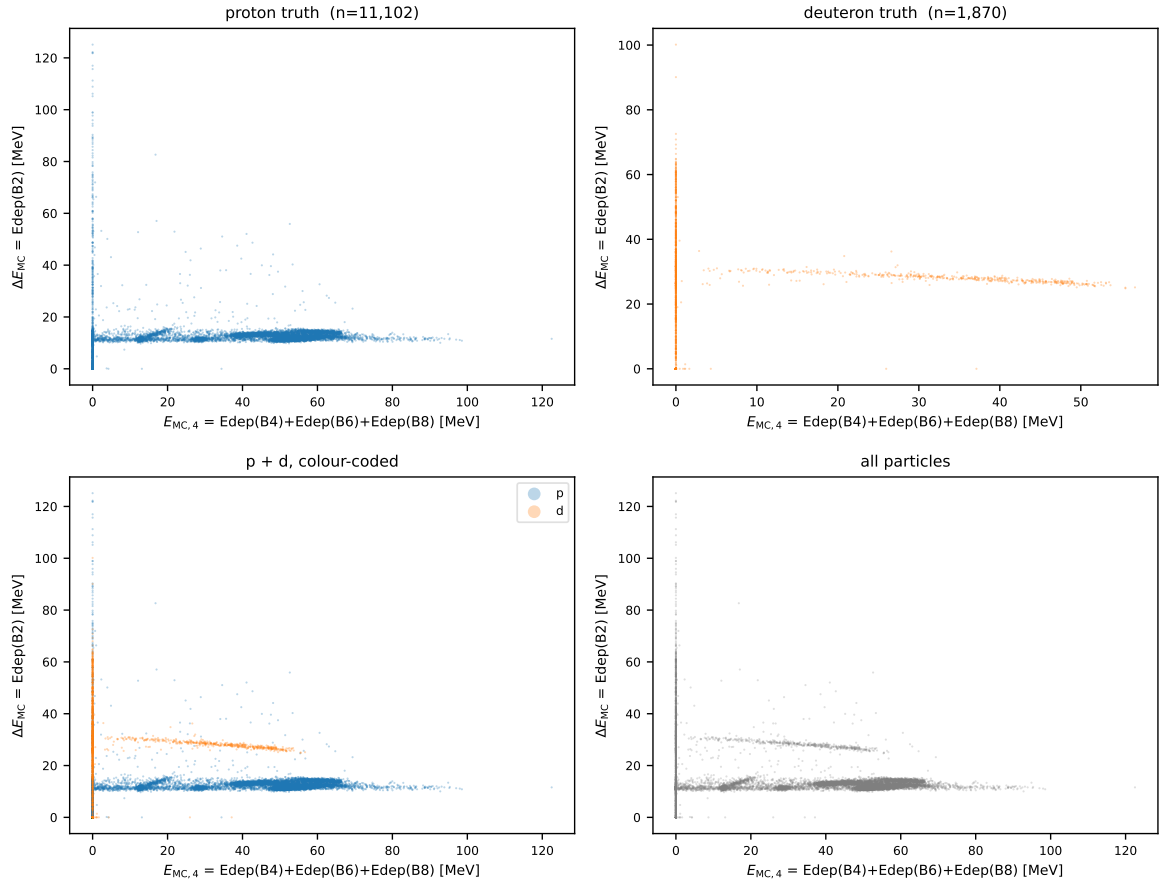
Figure 11: MC truth \Delta E -E, Sample II, data-matched four-layer definition (#618, SIMULATION_RESULT).
