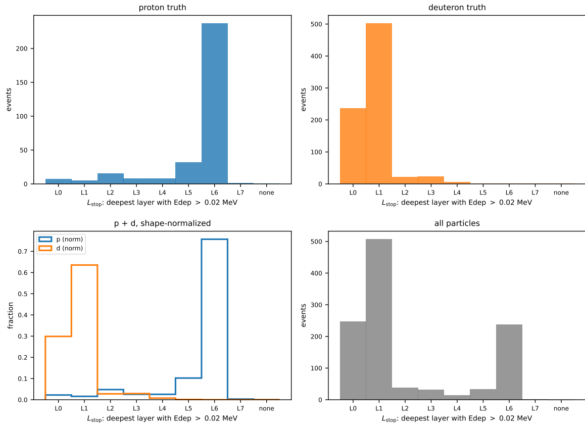
Figure 12: MC penetration depth L_{\text{stop}} , Sample I: proton, deuteron, shape-normalised overlay, all particles (#618, SIMULATION_RESULT).
