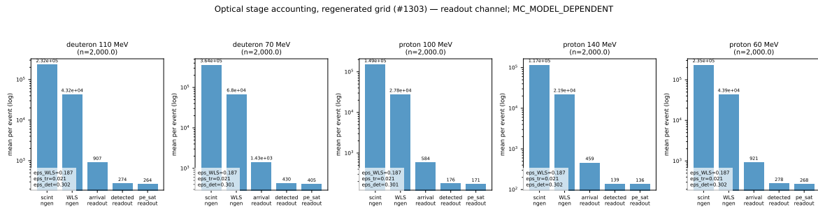
Figure 16: Regenerated five-point optical grid (#1303): stage-resolved accounting from scintillation production through WLS absorption/re-emission, guided transport, sensor arrival and detection to saturated-PE readout. Mean stage ratios: WLS capture \approx 0.19 , transport \approx 0.021 , detection-given-arrival \approx 0.30 , saturated-to-detected \approx 0.96 .
