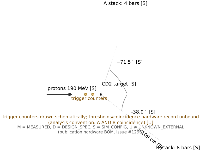
Figure 1: CCB two-arm geometry schematic. Beam energy, target, arm angles and bar counts are annotated on-figure with per-quantity evidence status from the hardware truth surface; they are simulation/configuration values, not survey-grade metrology.
