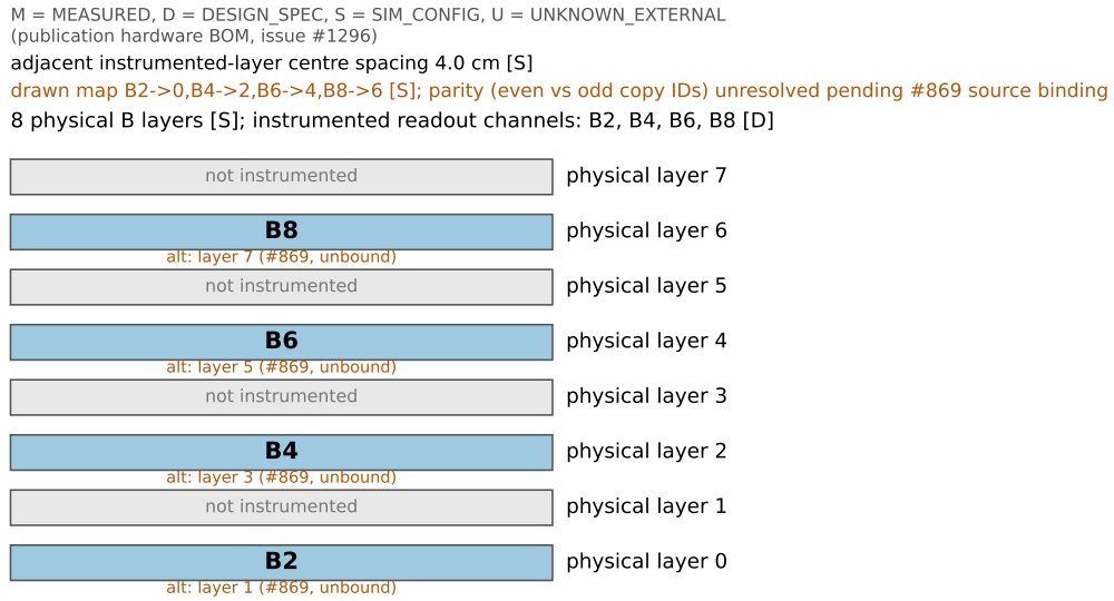
Figure 2: B-stack channel-to-layer correspondence. Channels B2/B4/B6/B8 sample every other physical Geant4 layer; the absolute offset between detector labels and copy IDs (the even-versus-odd parity of issue #869) is annotated as unresolved rather than silently chosen.
