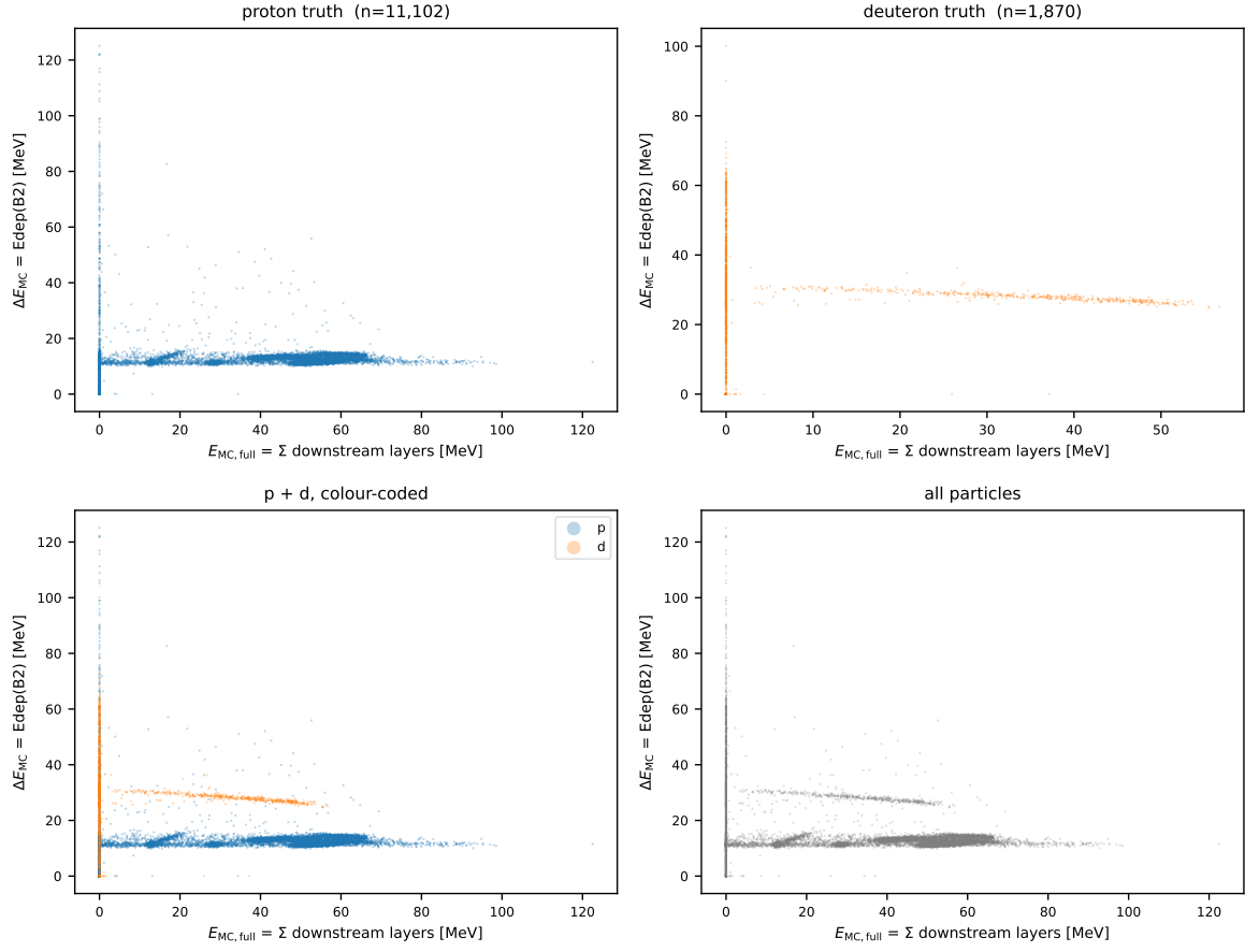
Figure 9: MC truth \Delta E - E , Sample II, full downstream sum; same panel structure (#618, SIMULATION_RESULT).
