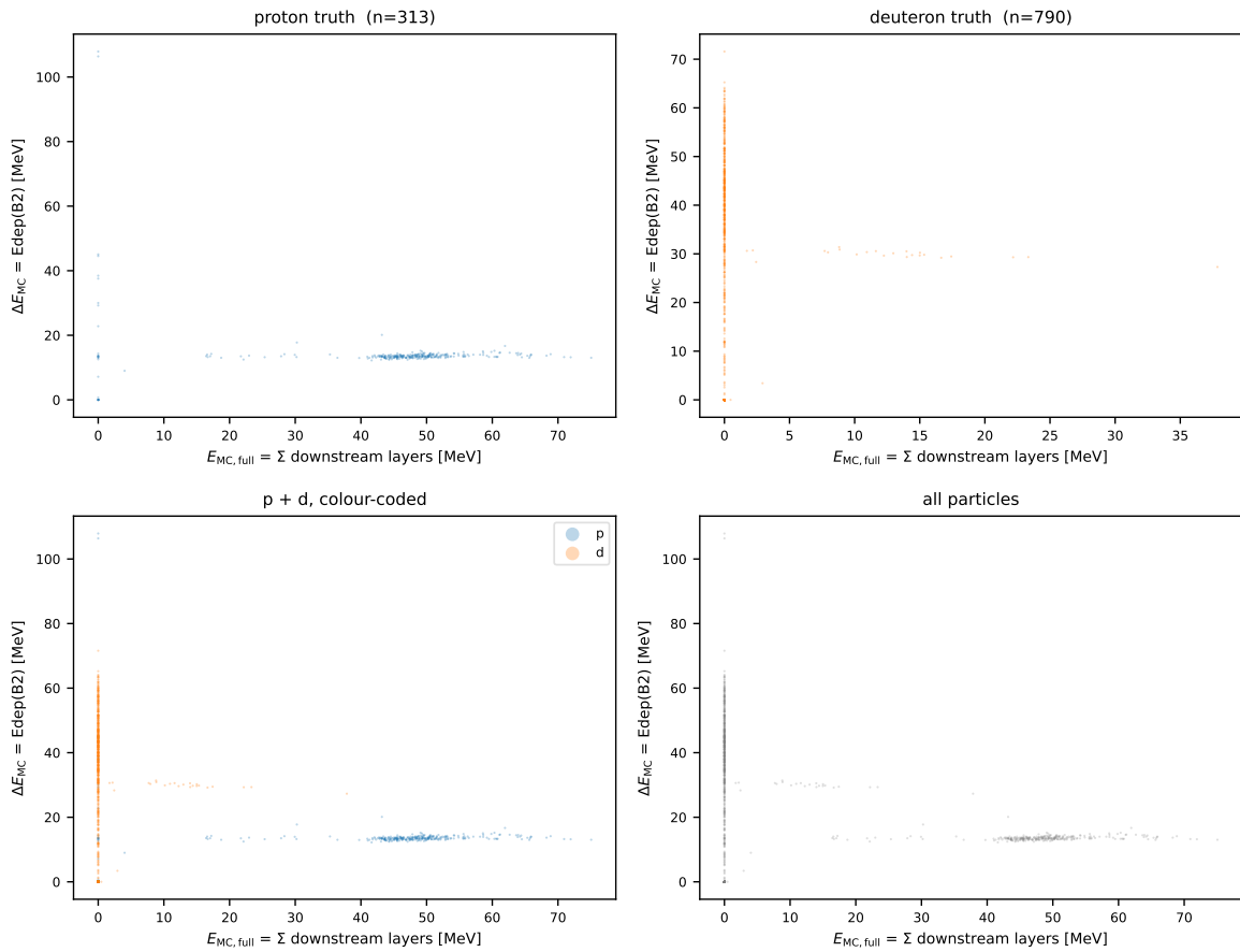
Figure 8: MC truth \Delta E - E , Sample I, full downstream sum; proton/deuteron/combined/all panels (#618, SIMULATION_RESULT ).
