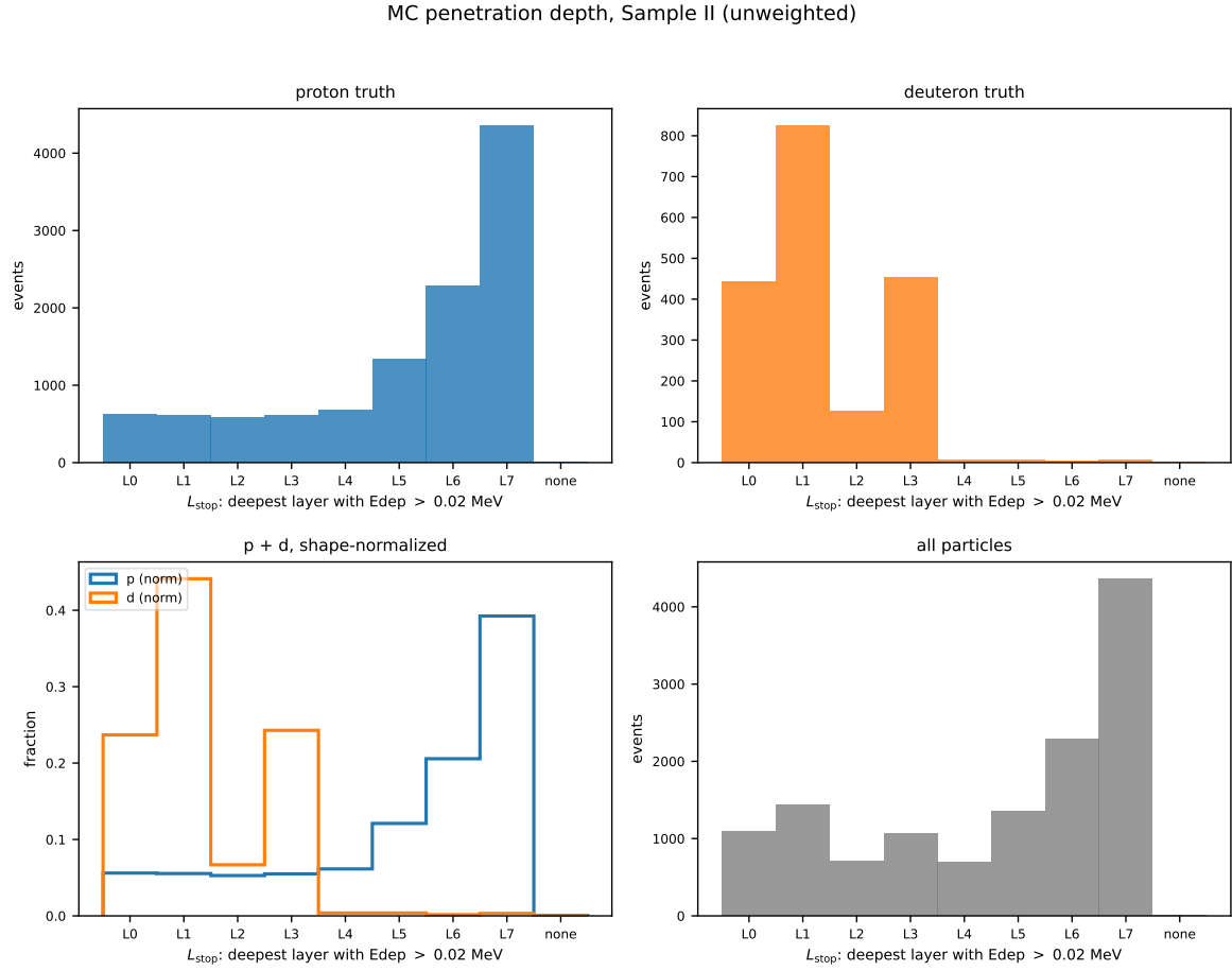
Figure 13: MC penetration depth L_{\text{stop}} , Sample II, same panel structure (#618, SIMULATION_RESULT).
