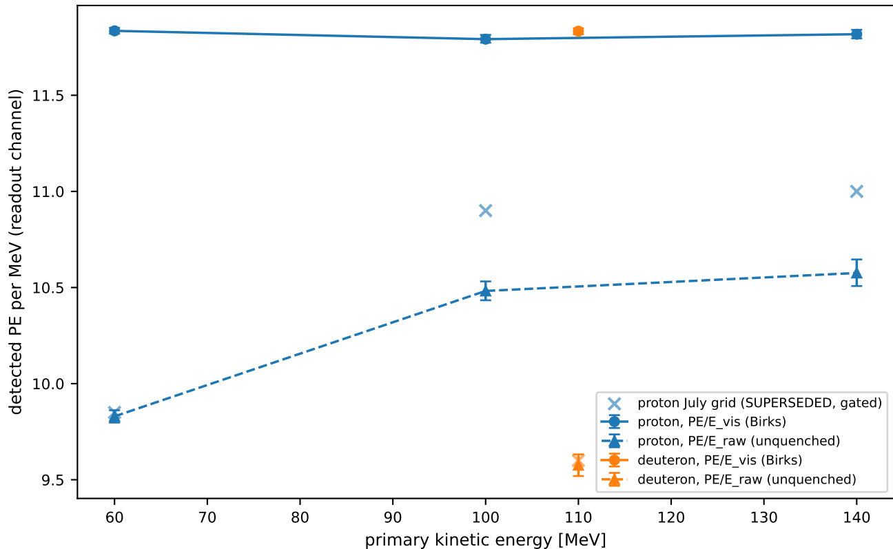
Regenerated light-collection scale vs July grid (#1303); 68% bootstrap CIs; MC_MODEL_DEPENDENT
