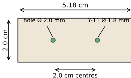
(b) transverse cross-section (to scale)
