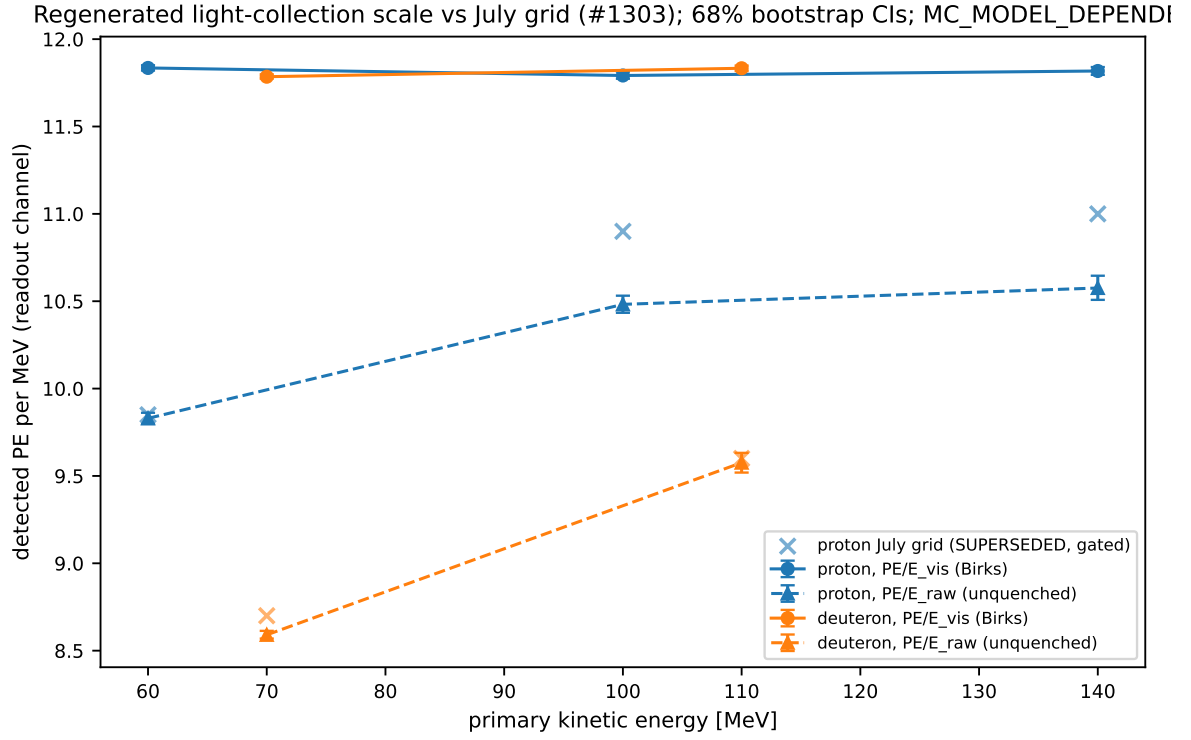
Figure 17: Per-point detected-PE yields per visible MeV (flat within bootstrap intervals, 11.78–11.84) and per raw deposited MeV (8.6–10.6, species-split through the Birks quenching ratio) across the five-point grid (#1303).
