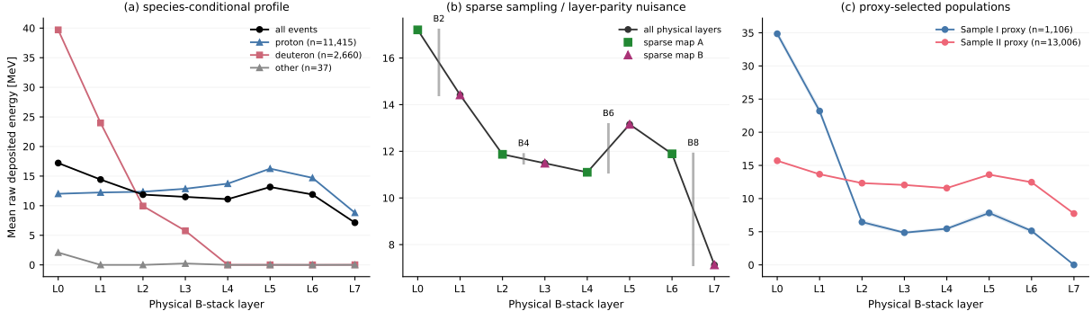
Figure 5: MC longitudinal deposited-energy profile of the proxy-selected population ( n = 14,112 , weights verified unit, ESS = 14,112): (a) per-layer mean raw deposited energy, species-resolved, with event-bootstrap 16–84% bands on the total; (b) the sparse B2/B4/B6/B8 sampling of the same profile under both parity hypotheses of issue #869, drawn as a nuisance envelope because the channel-to-layer offset is unresolved (neither the BOM even map #1296 nor the legacy odd map carried by the #618 readout columns is canonical); (c) the proxy Sample I/II populations. Energy is raw deposited MeV, not Birks-visible (#1302).
