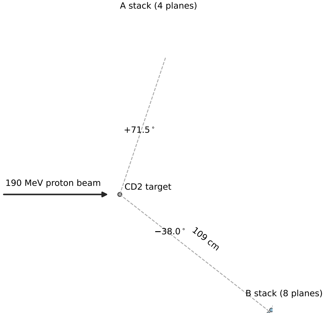
Figure 1: CCB two-arm geometry schematic. Beam energy, target, arm angles and bar counts are annotated on-figure with per-quantity evidence status from the hardware truth surface; they are simulation/configuration values, not survey-grade metrology.
