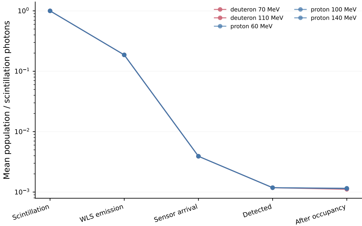
Figure 16: Regenerated five-point optical grid (#1303): stage-resolved accounting from scintillation production through WLS absorption/re-emission, guided transport, sensor arrival and detection to saturated-PE readout. Mean stage ratios: WLS capture \approx 0.19 , transport \approx 0.021 , detection-given-arrival \approx 0.30 , saturated-to-detected \approx 0.96 .
