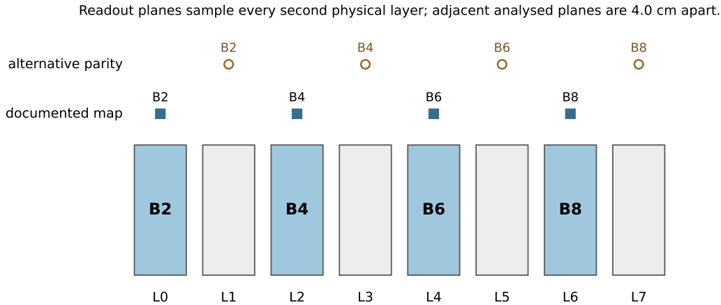
Figure 2: B-stack channel-to-layer correspondence. Channels B2/B4/B6/B8 sample every other physical Geant4 layer; the absolute offset between detector labels and copy IDs (the even-versus-odd parity of issue #869) is annotated as unresolved rather than silently chosen.
