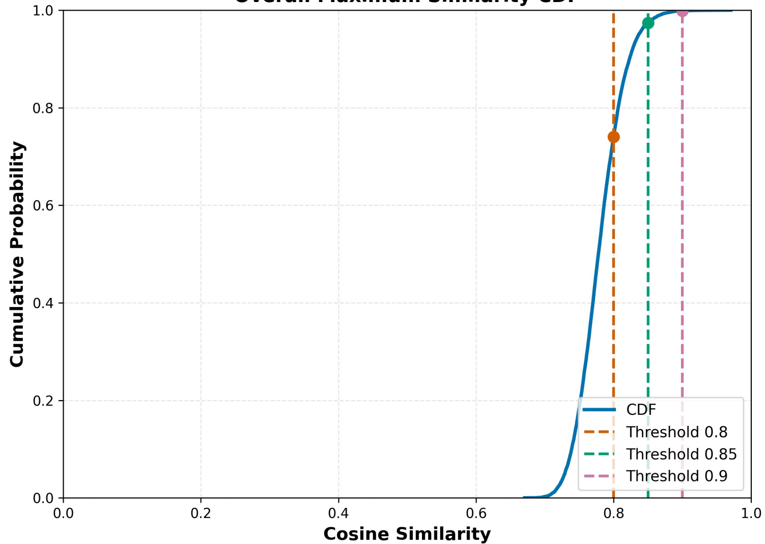
Overall Maximum Similarity CDF
