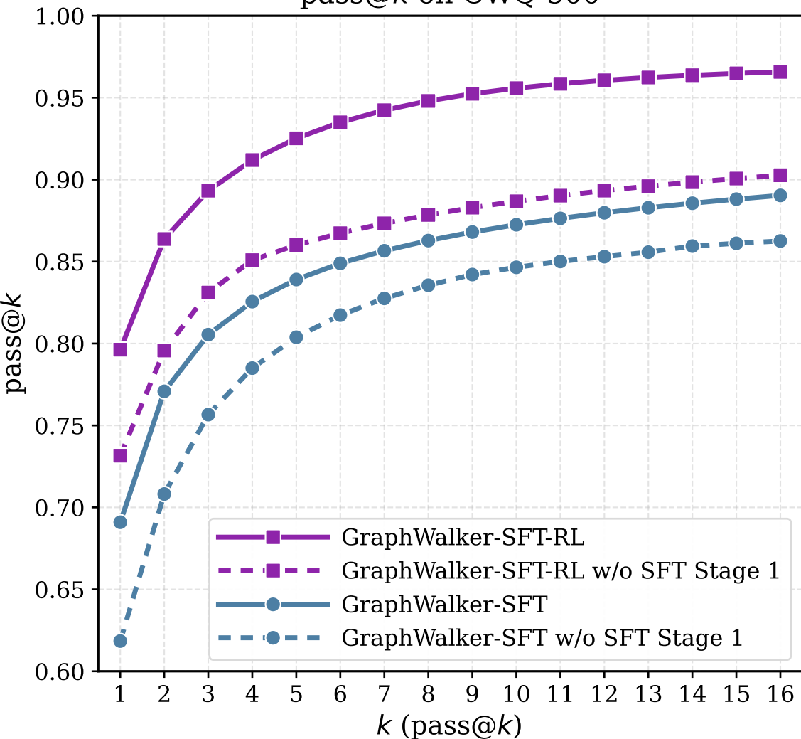
pass@k on CWQ-500
