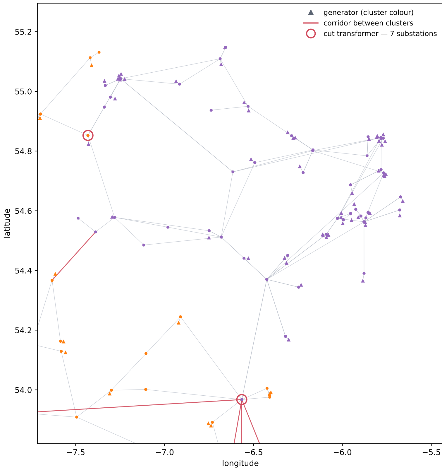
WP2024_all-island +generators — sym, headroom, k = 6, 2030-01-20 17:00:00 cluster 4 — 171 nodes
