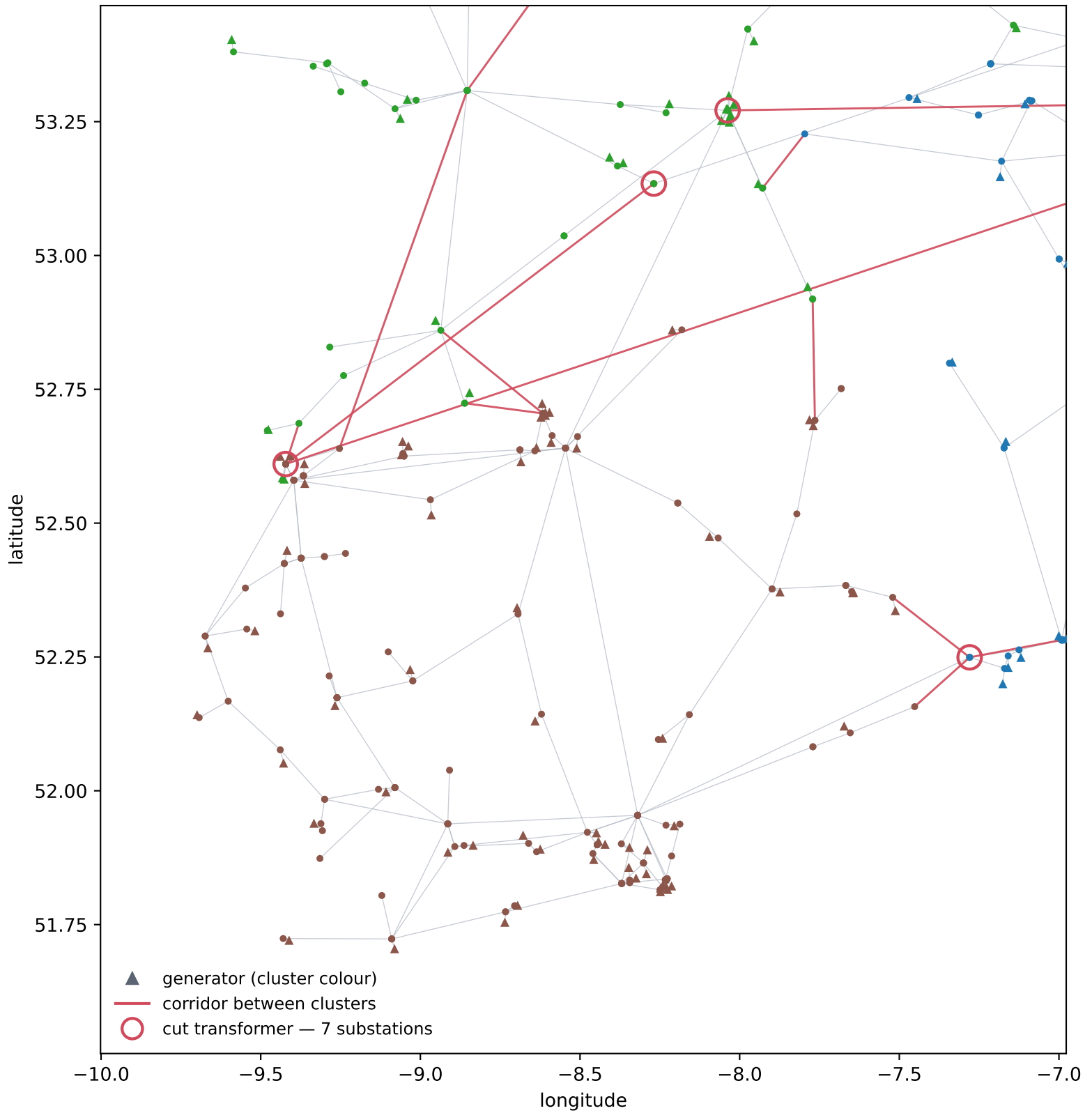
WP2024_all-island +generators — sym, headroom, k = 6, 2030-01-20 17:00:00 cluster 5 — 225 nodes
