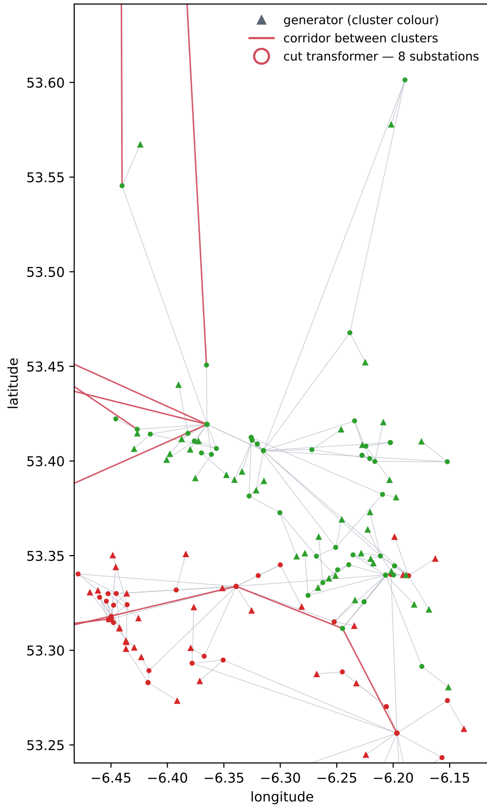
WP2024_all-island +generators — sym, loading, k = 6, 2030-01-20 17:00:00 cluster 2 — 108 nodes
