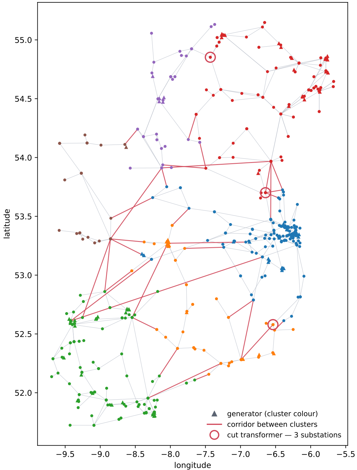
TYTFS2024_WP2024_V35_transmission +generators — sym, susceptance, k = 6 643/643 buses placed, 35/895 drawn corridors cut
