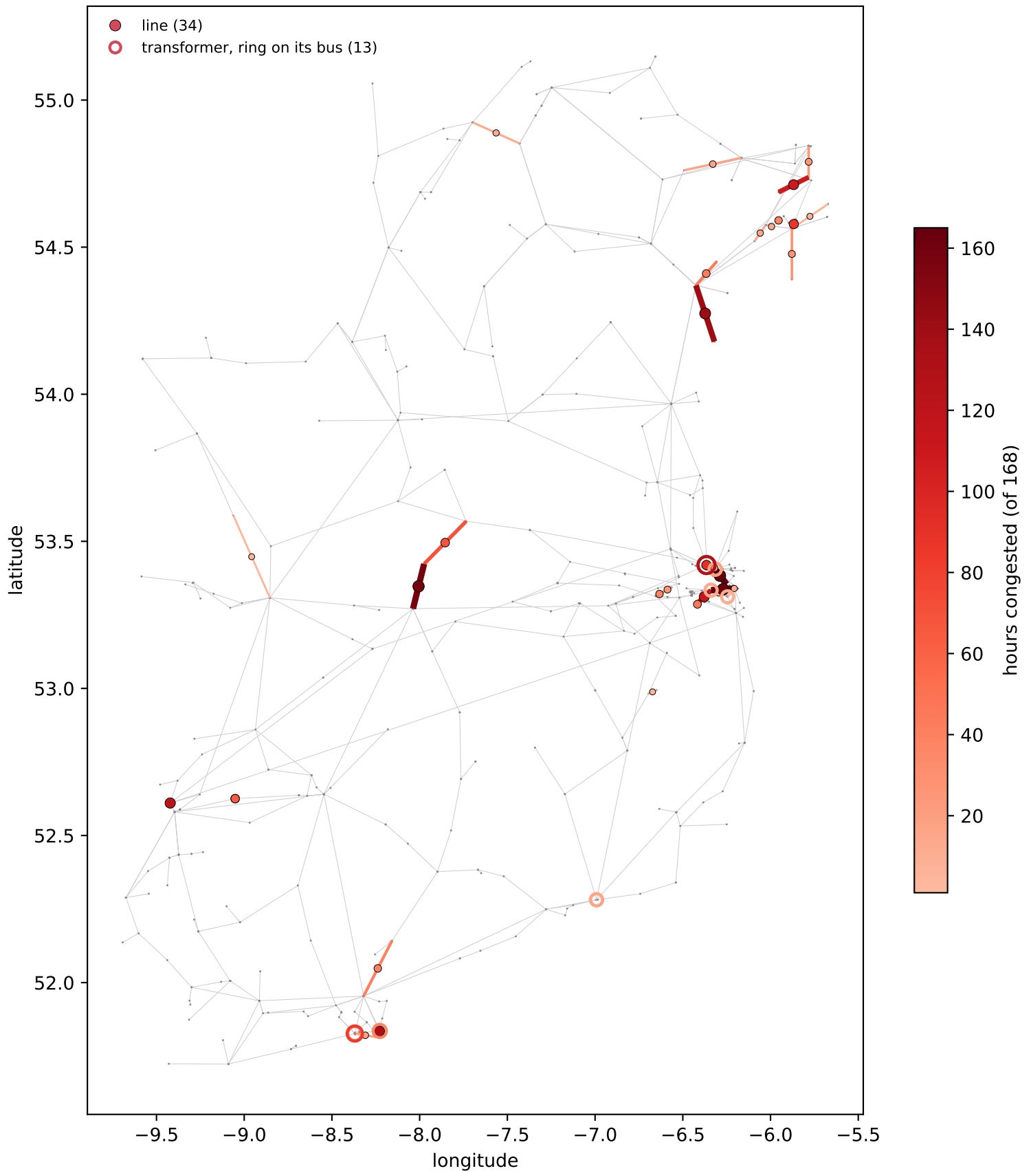
WP2024_all-island (prorata) - branches at \geq 50\% of rating, over 168 hours 47 of 848 branches congested at least once; 0 of them not placeable
