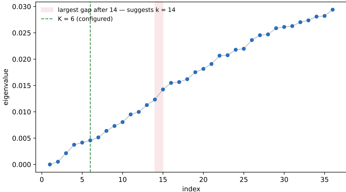
WP2024_all-island +generators — sym, loading
