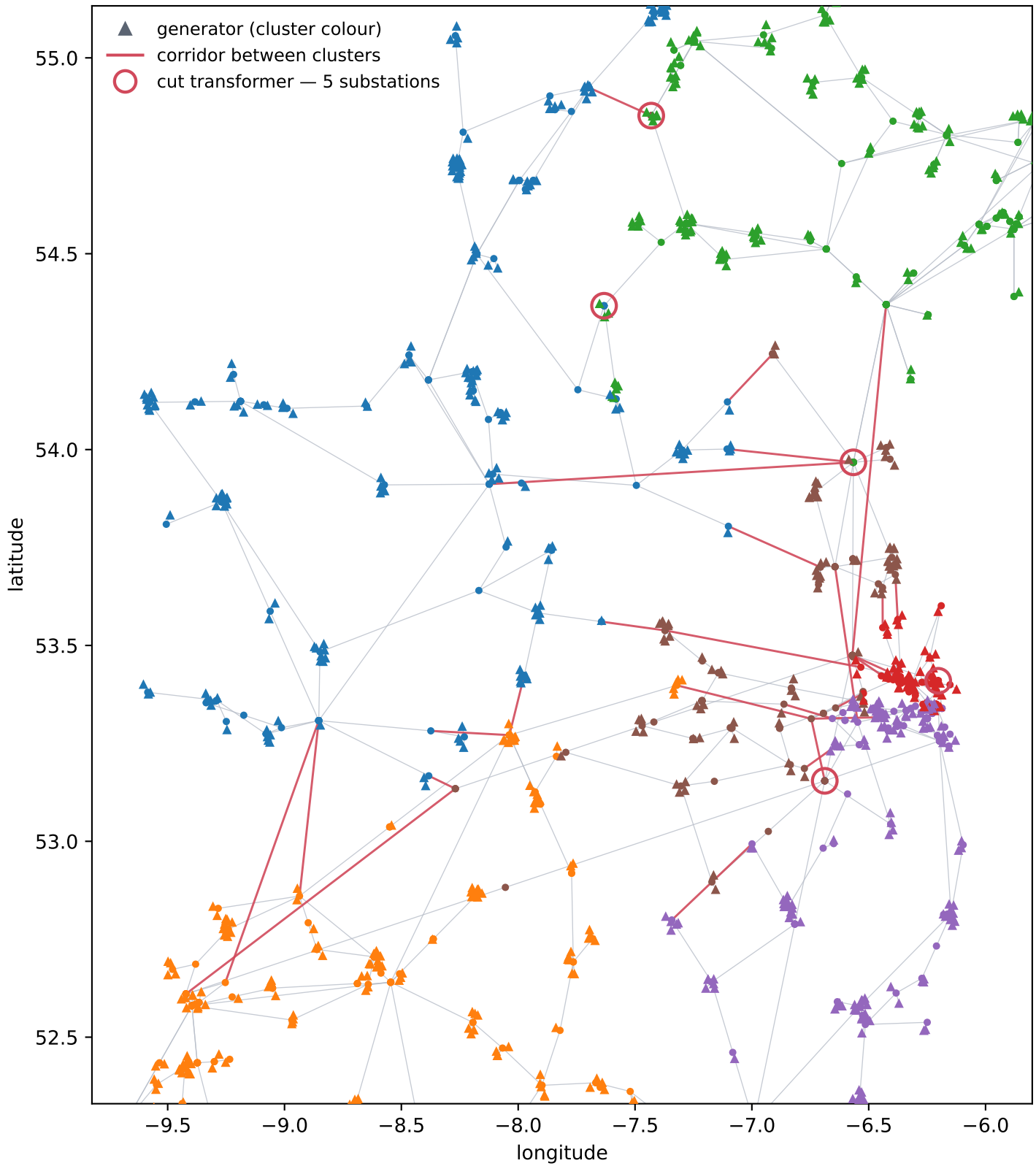
WP2033_all-island +generators — sym, headroom, k = 6, 2030-01-20 17:00:00 cluster 5 — 182 nodes
