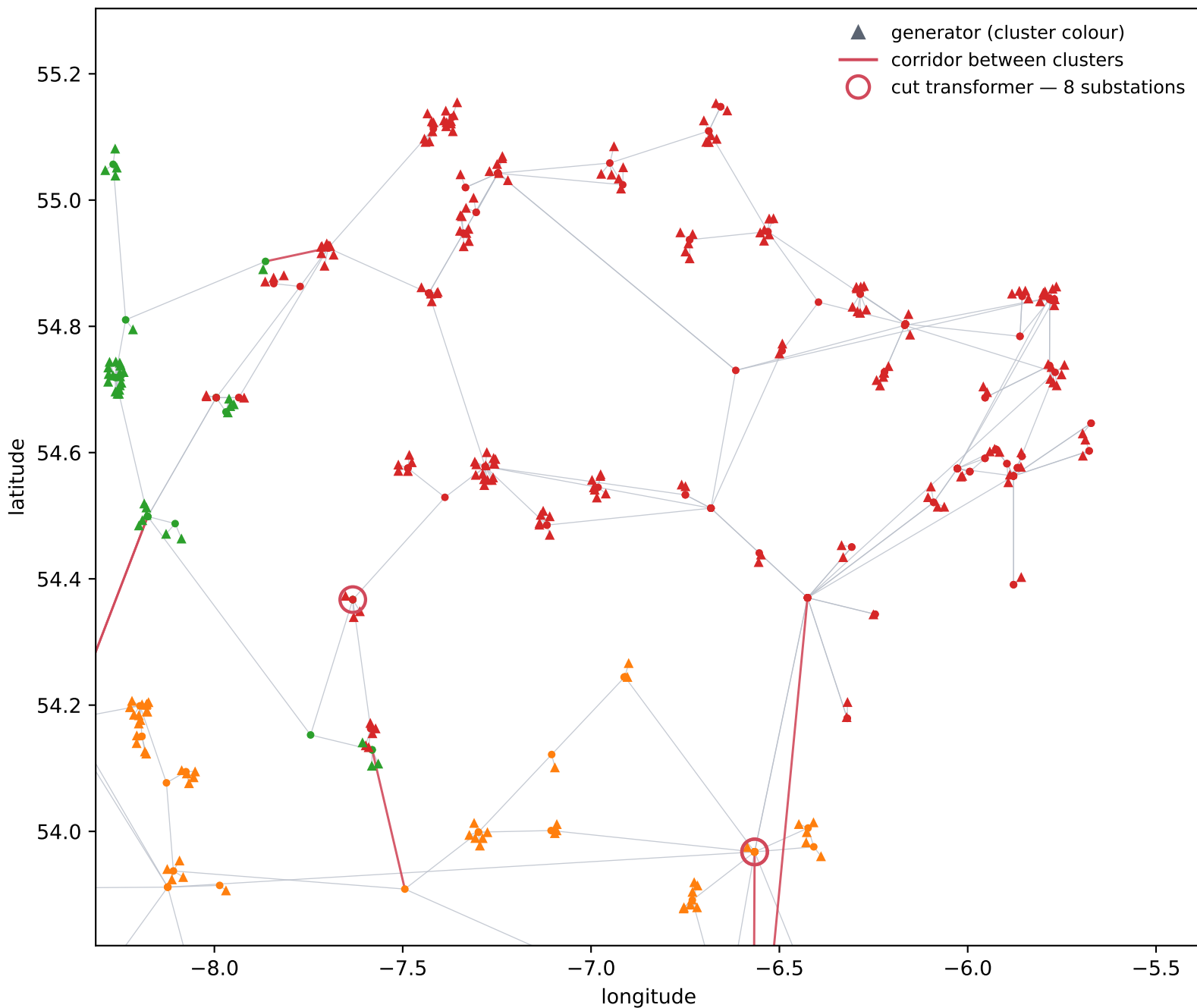
WP2033_all-island +generators — sym, loading, k = 6, 2030-01-20 17:00:00 cluster 3 — 335 nodes
