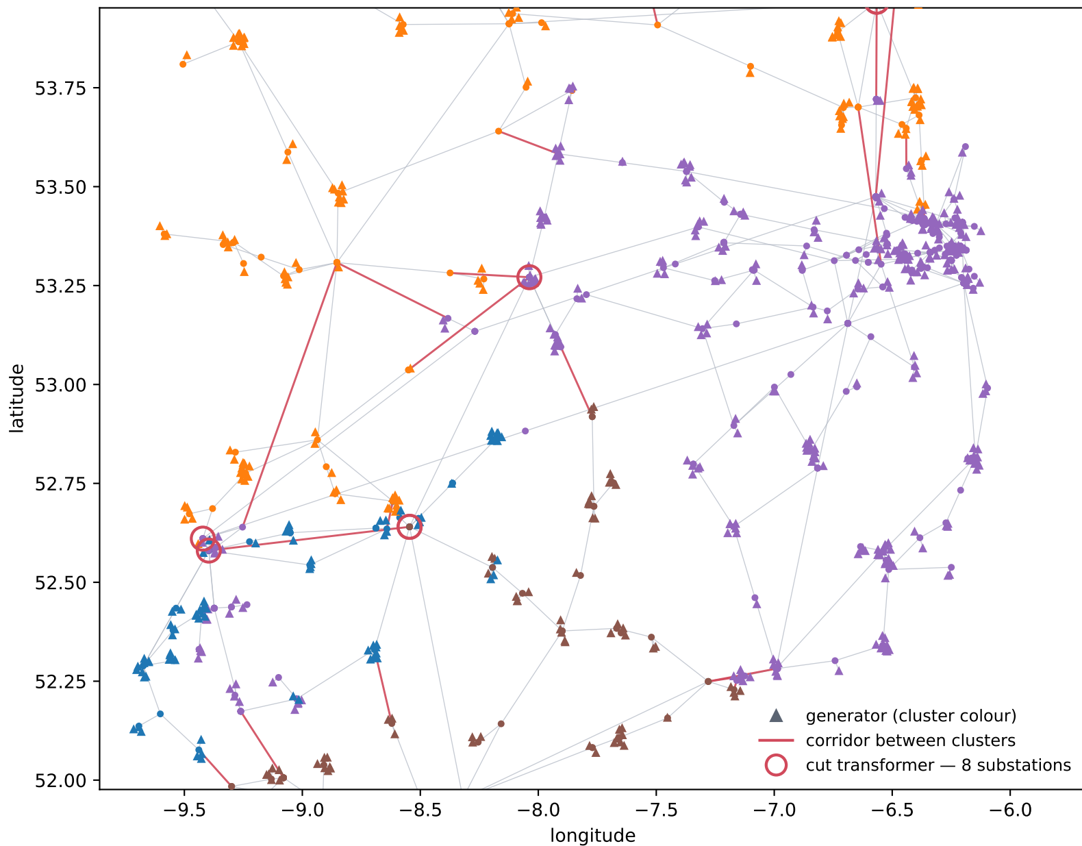
WP2033_all-island +generators — sym, loading, k = 6, 2030-01-20 17:00:00 cluster 4 — 624 nodes
