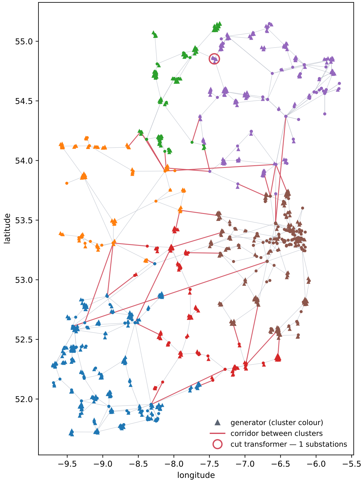
TYTFS2024_WP2033_V35_transmission +generators — sym, susceptance, k = 6 746/751 buses placed, 35/1637 drawn corridors cut
