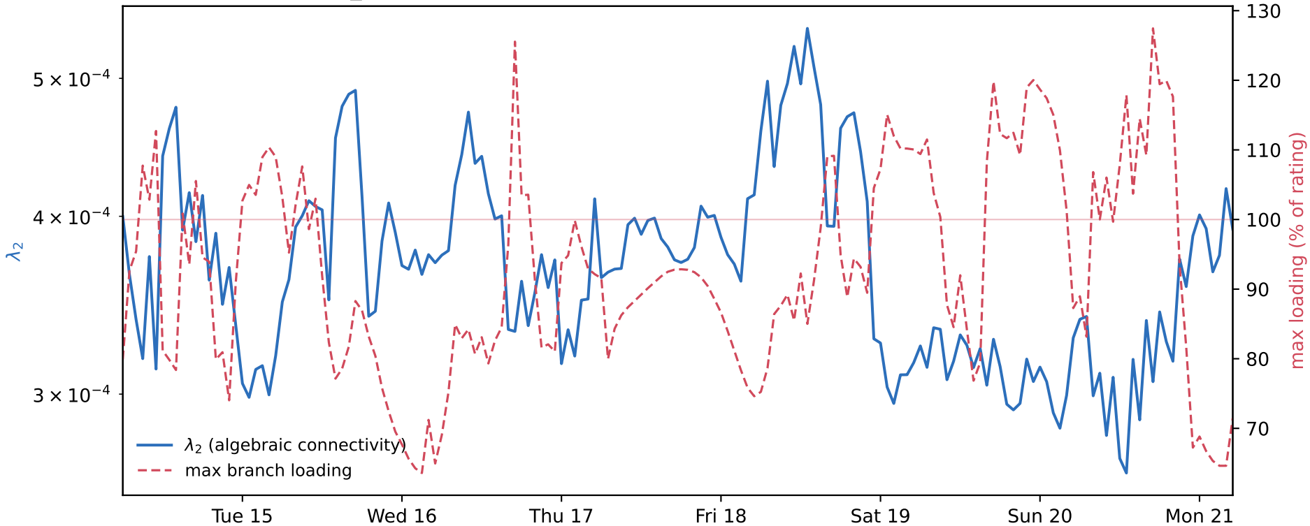
WP2033_all-island - loading: how close the grid is to splitting, hour by hour
