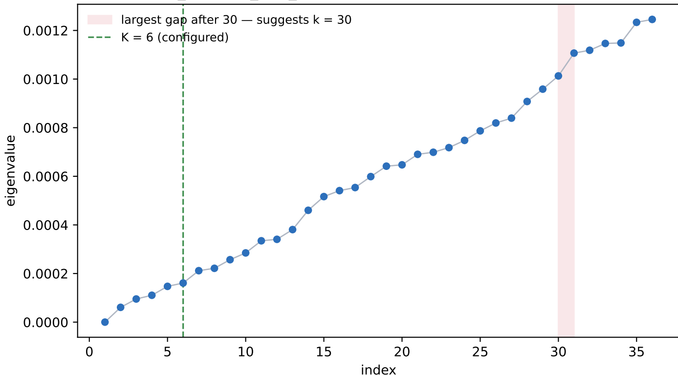
TYTFS2024_WP2033_V35_transmission +generators — sym, susceptance
