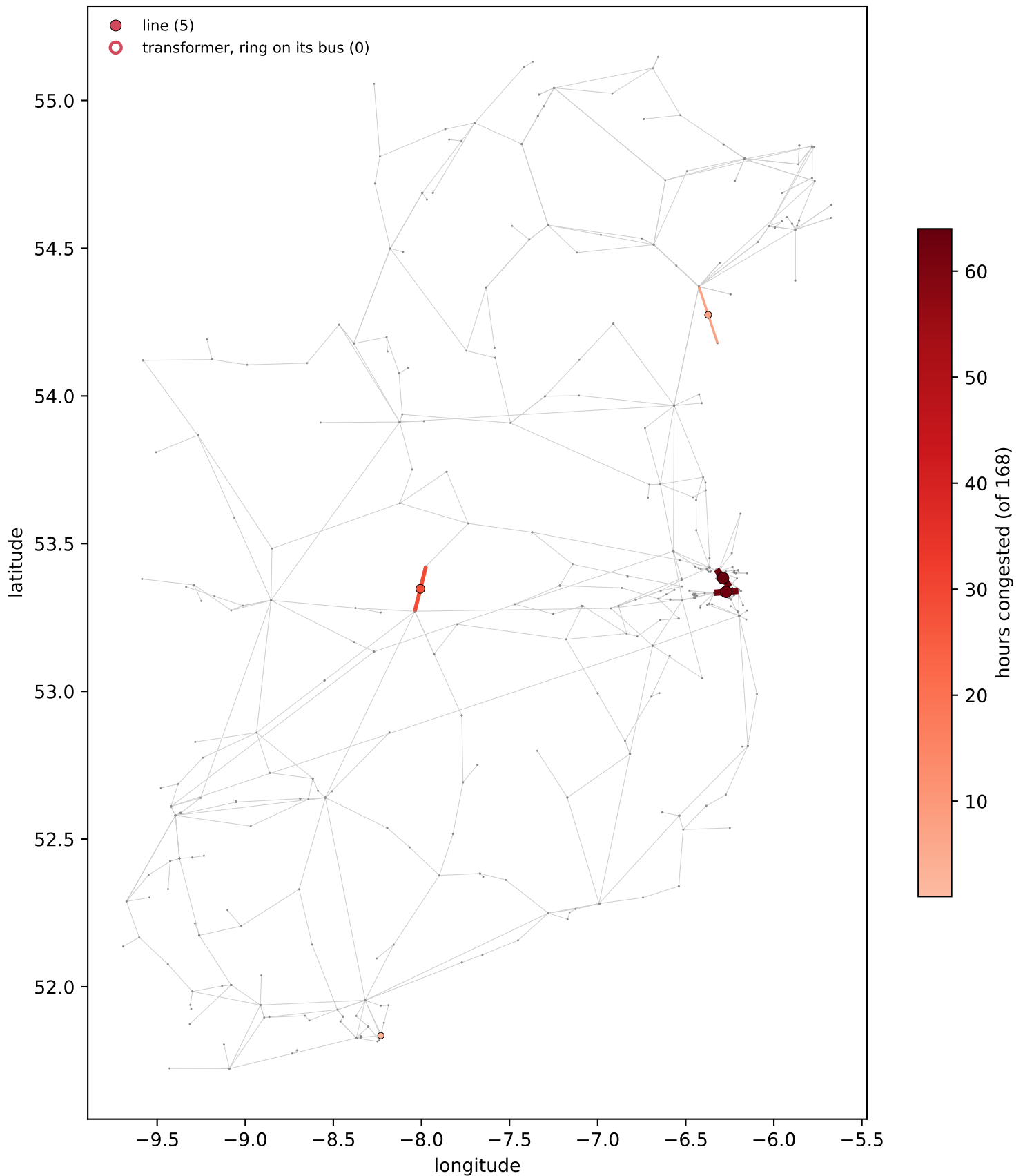
WP2024_all-island (prorata) - branches at \geq 70\% of rating, over 168 hours 5 of 848 branches congested at least once; 0 of them not placeable
