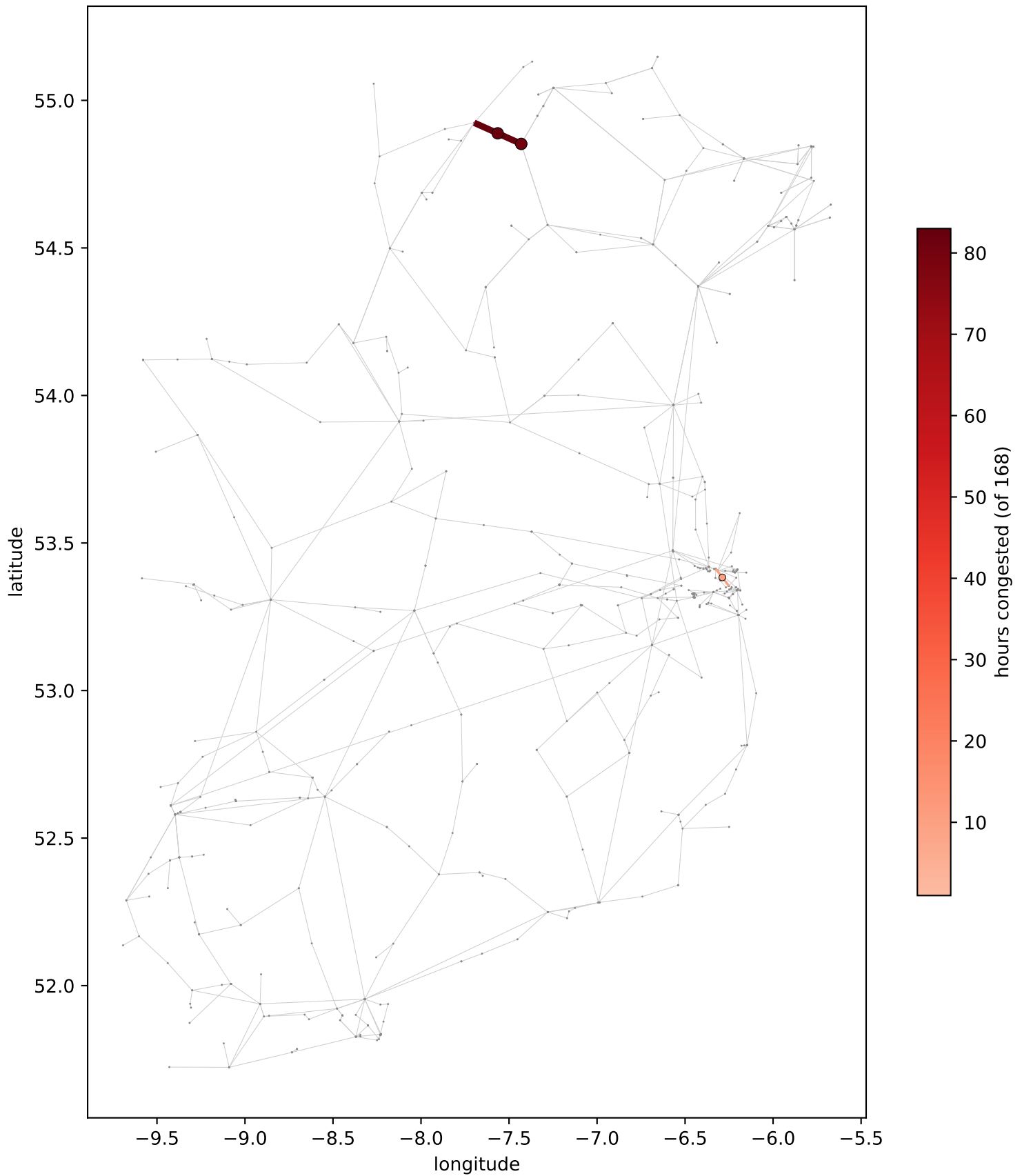
WP2033_all-island - branches at \geq 90\% of rating, over 168 hours 4 of 980 branches congested at least once; 0 of them not placeable
