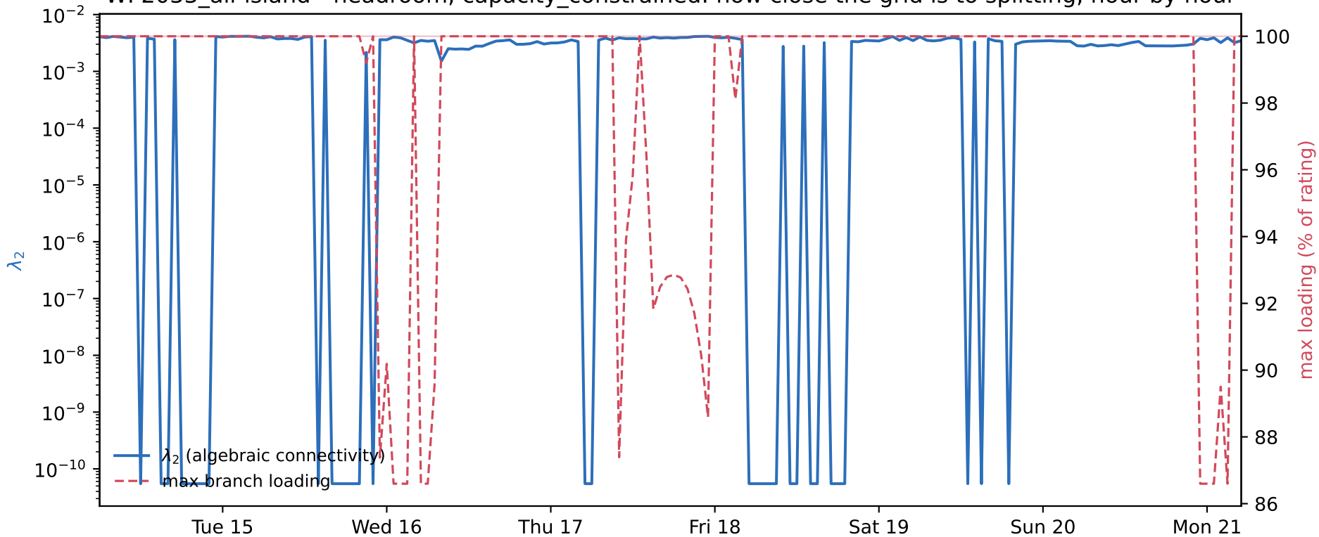
WP2033_all-island - headroom, capacity_constrained: how close the grid is to splitting, hour by hour
