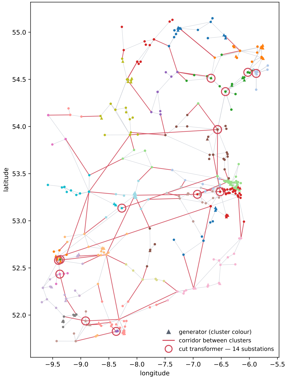
TYTFS2024_WP2024_V35_transmission +generators — sym, susceptance, k = 33 643/643 buses placed, 103/895 drawn corridors cut
